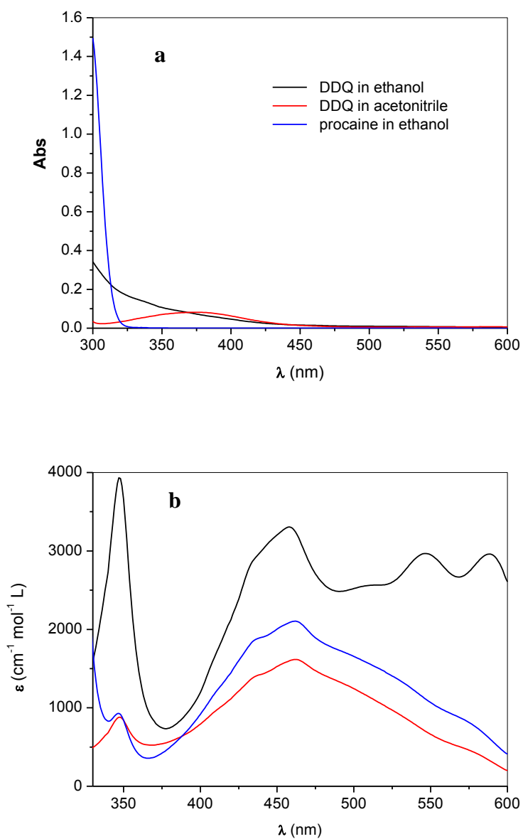
Figure 7. a) Spectra of the single components of the solutions 1 \cdot 10^{-4} \text{ mol L}^{-1} . The spectra of atenolol are not reported because it does not absorb in the range 300-600 nm. b) Absorption spectra of the complexes DDQ-procaine (blue: in ethanol) and DDQ-atenolol (red: in ethanol; black: in acetonitrile), calculated with HypSpec®.
