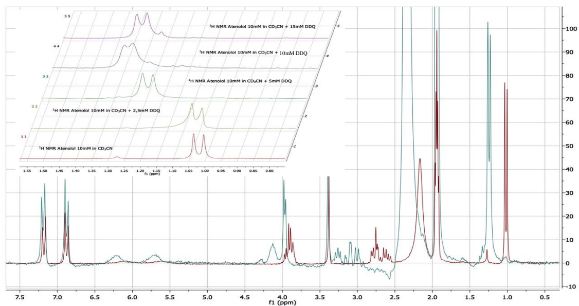
Figure 9. ^1\text{H-NMR} spectra of the drug in acetonitrile- \text{d}_3 , before and after the addition of 0.5 eq of DDQ: Atenolol 10.0 \text{ mmol L}^{-1} (red), Atenolol 10.0 \text{ mmol L}^{-1} and DDQ 5.0 \text{ mmol L}^{-1} (blue); nested graph: ^1\text{H-NMR} \text{CH}_3 -region shift observed during titration.
