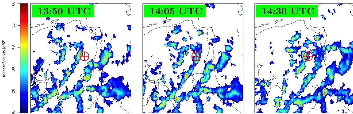
Figure 8. Same as Figure 6 for 26 August 2012 when there were three events measured. Event #6 was measured at 13:52:23 UTC, Event #7 at 14:02:56 UTC, and Event #8 at 14:28:19 UTC.
