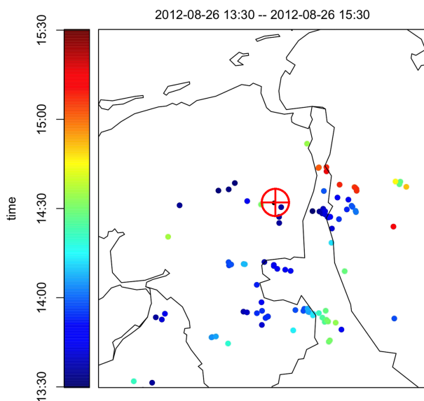
Figure 7. Lightning discharges on 26 August 2012 between 13:30 and 15:30 UTC as indicated by the color of the points. The red ⊕ gives the location of LOFAR “Superterp.” There were three events measured on this day. Event #6 was measured at 13:52:23 UTC, Event #7 at 14:02:56 UTC, and Event #8 at 14:28:19 UTC. Data from KNMI (2018).
