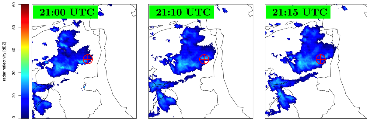
Figure 6. Radar reflectivity in dBz as determined for different UTC times on 14 December 2011. The red ⊕ marks the location of the LOFAR “Superterp.” There were three events measured on this day. Event #1 was measured at 21:02:27 UTC, Event #2 at 21:10:01 UTC, and Event #3 at 21:14:34 UTC. Each picture shows an area of about 160 × 180 km 2 . Data from ADAGUC (2018).
