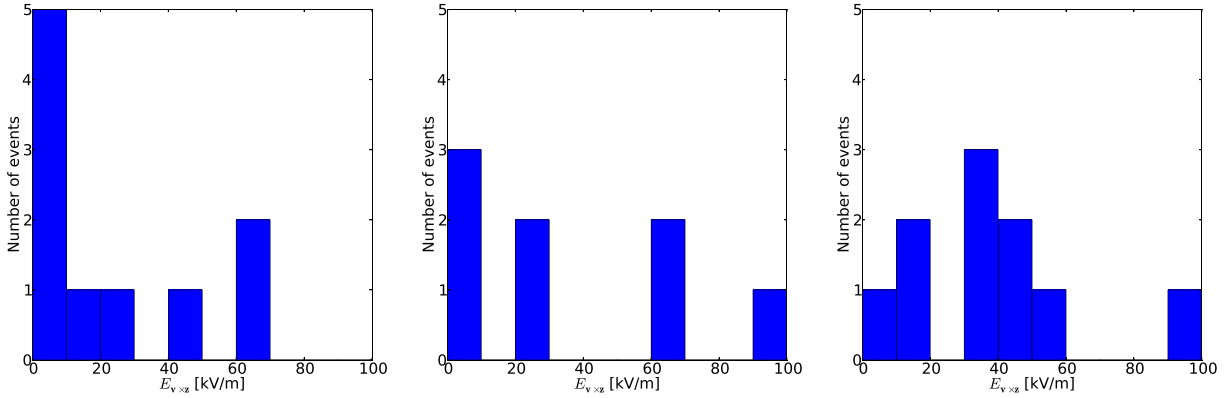
Figure 10. E_{v_{xz}} distribution, left: bottom layer, middle: middle layer, and right: top layer.
