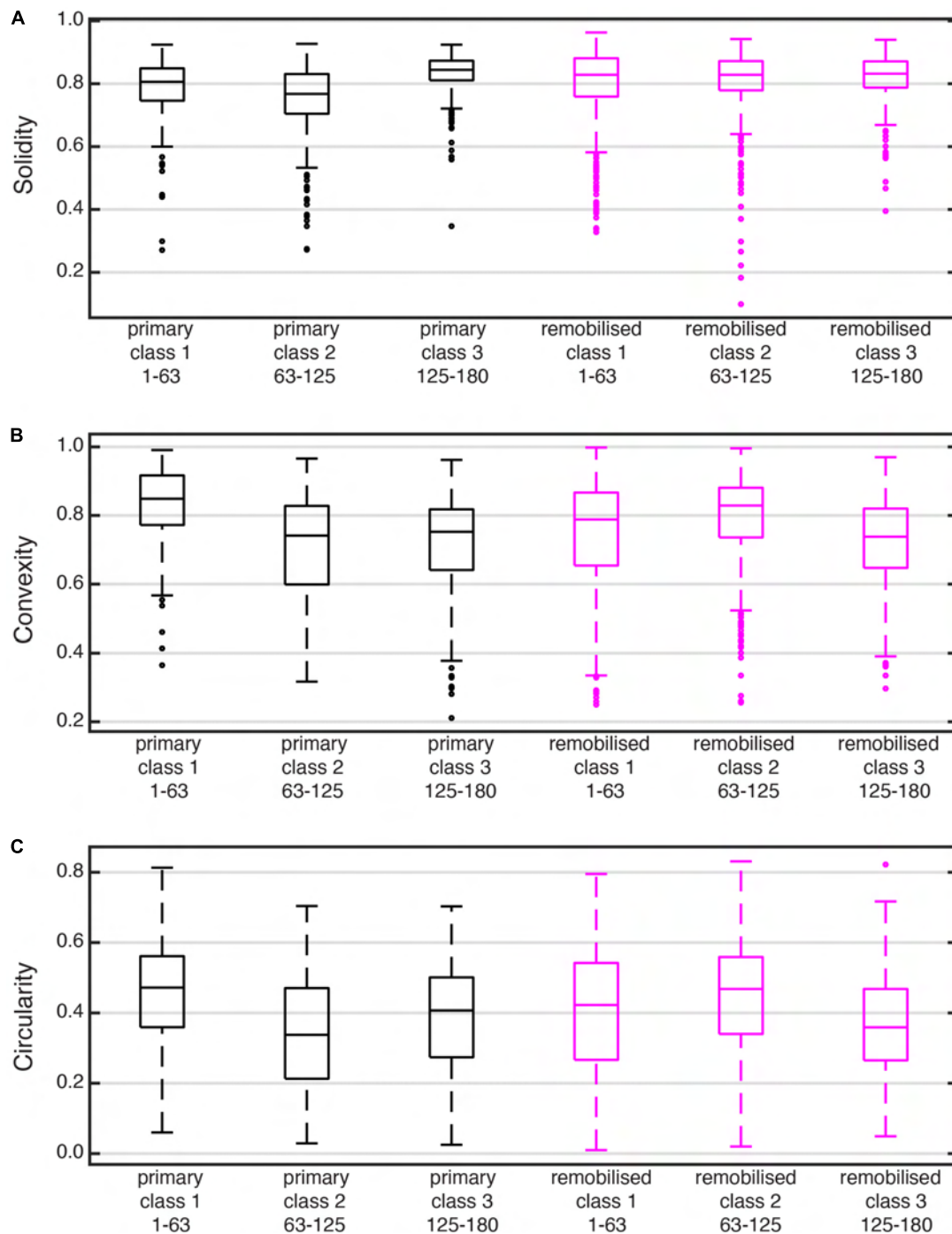
FIGURE 9 | Box and whisker plots showing comparison of (A) solidity, (B) convexity, and (C) circularity for primary and remobilised ash. The three parameters are dimensionless and scaled from 0 to 1, being 1 the perfect circle. Lower and upper edges of each box indicate the 25 and 75% percentiles, respectively, with the middle line corresponding to the median. Box width represents the variability of values within the same sample. The whiskers extend to the most extreme values and the points correspond to outliers.
