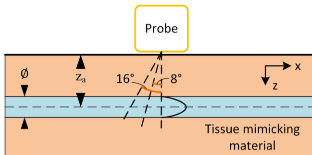
Fig. 2. Schematic of the experimental and simulation set-up.
