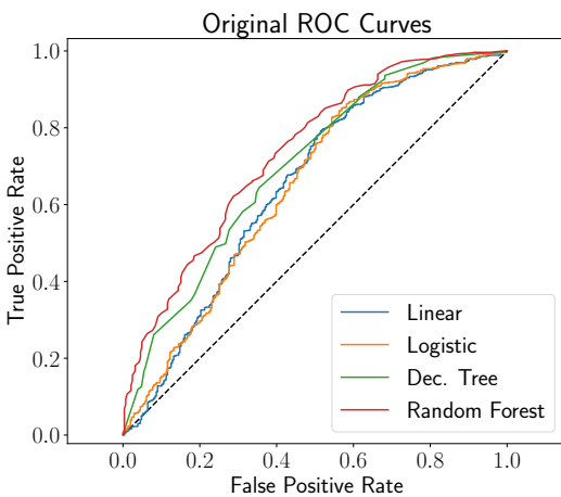
Figure 9. ROC curves for models trained on original variables
