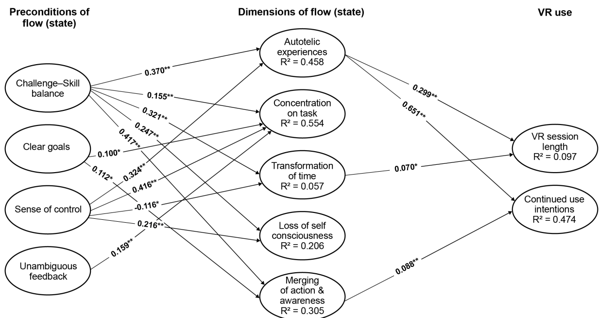
Figure 2: Results: * = p < 0.1, ** = p < 0.05. (Non-significant paths omitted for clarity. See Table 3 for all path coefficients)
