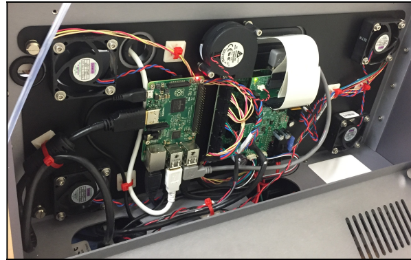
Figure 1: Rear Compartment of the Voxel8
