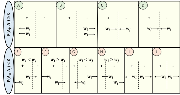
Figure 2. A comprehensive overview of URMC algorithm.
