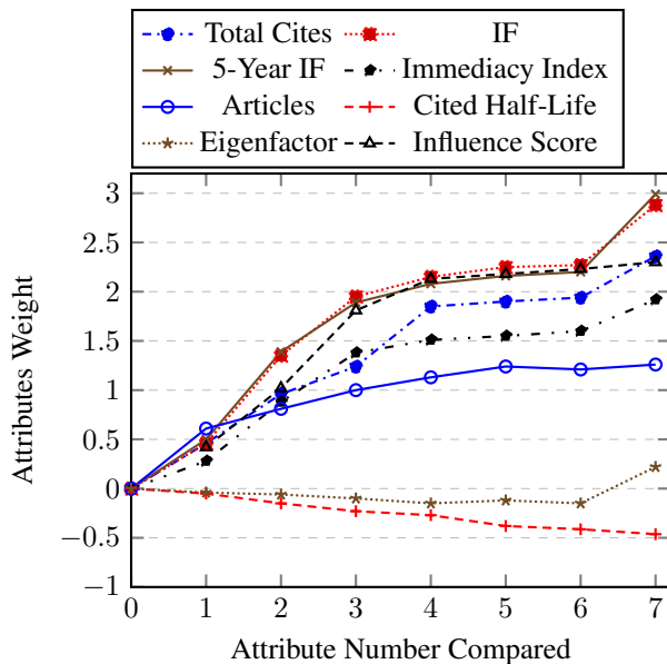
Figure 4. How attribute weights change using Algorithm 1 on the JR dataset with eight attributes.
