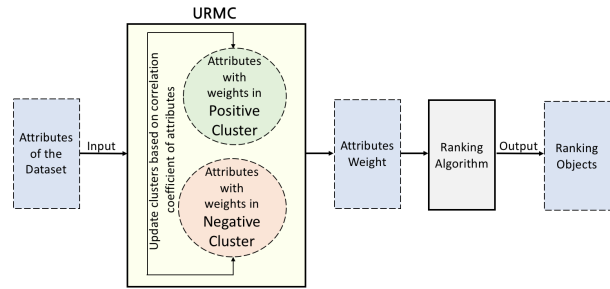
Figure 1. High-level depiction of the steps for unsupervised ranking of multi-attribute objects.
