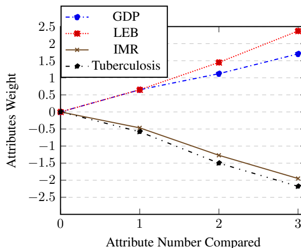
Figure 6. How attribute weights change using Algorithm 1 on the LQC dataset.
