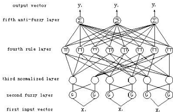
Fig.1 normalized neural network analysis structure
