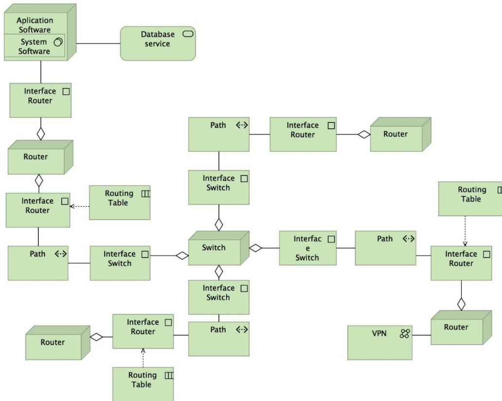
Figure 9 Infrastructure of an IXP model in Archi.
