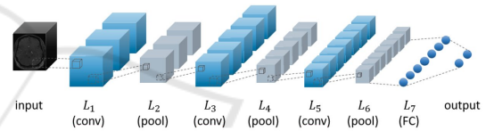
Figure 2: Illustration of the convolutional neural network used in this paper. The architecture consists of three convolutional ( L_1, L_3, L_5 ) and three max pooling ( L_2, L_4, L_6 ) layers followed by a fully connected ( L_7 ) layer.
