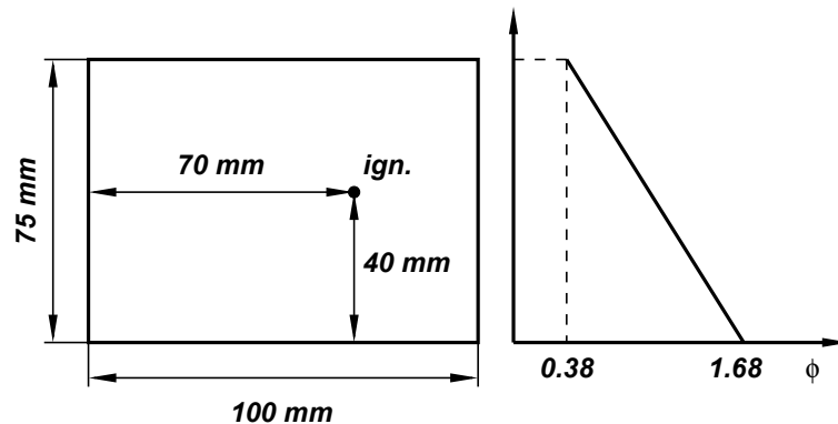
Figure 7: Sketch of the geometry and the initial equivalence ratio distribution in the case 2 of the two-dimensional combustion bomb test.
