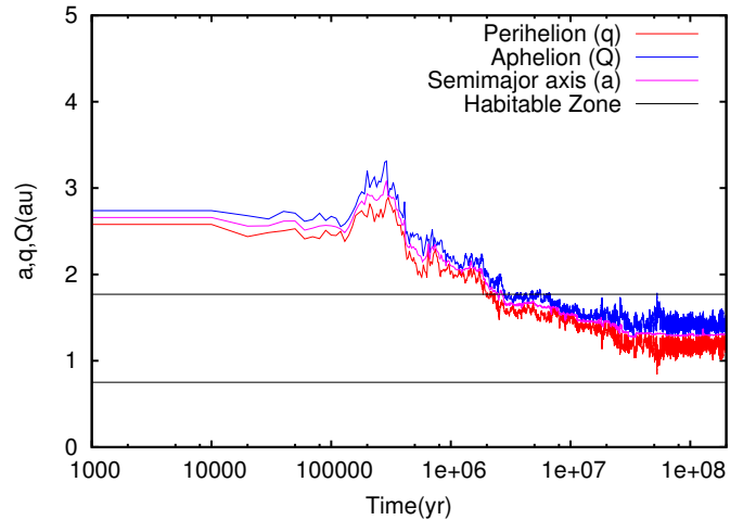
Fig. 14. Evolution in time of the semimajor axis a , and the perihelion q and aphelion Q distances of the super-Earth that survived in the HZ in SIM 1 corresponding to scenario IV. The black lines indicate the limits of the optimistic HZ.
