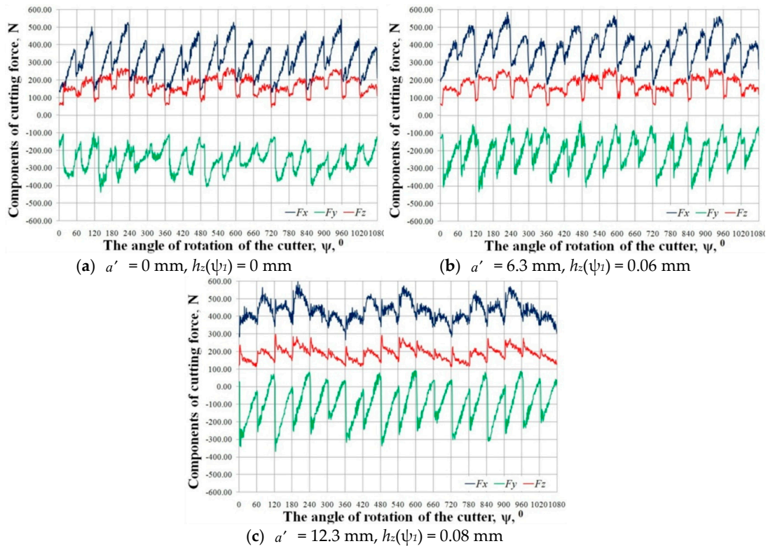
Figure 3. The cutting force components' time courses.
