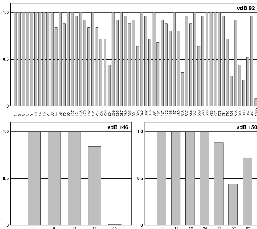
Figure 4. Histogram showing the probability in which a cluster member previously determined keeps its membership condition throughout the 25 simulations for vdB92, vdB146 and vdB150.
