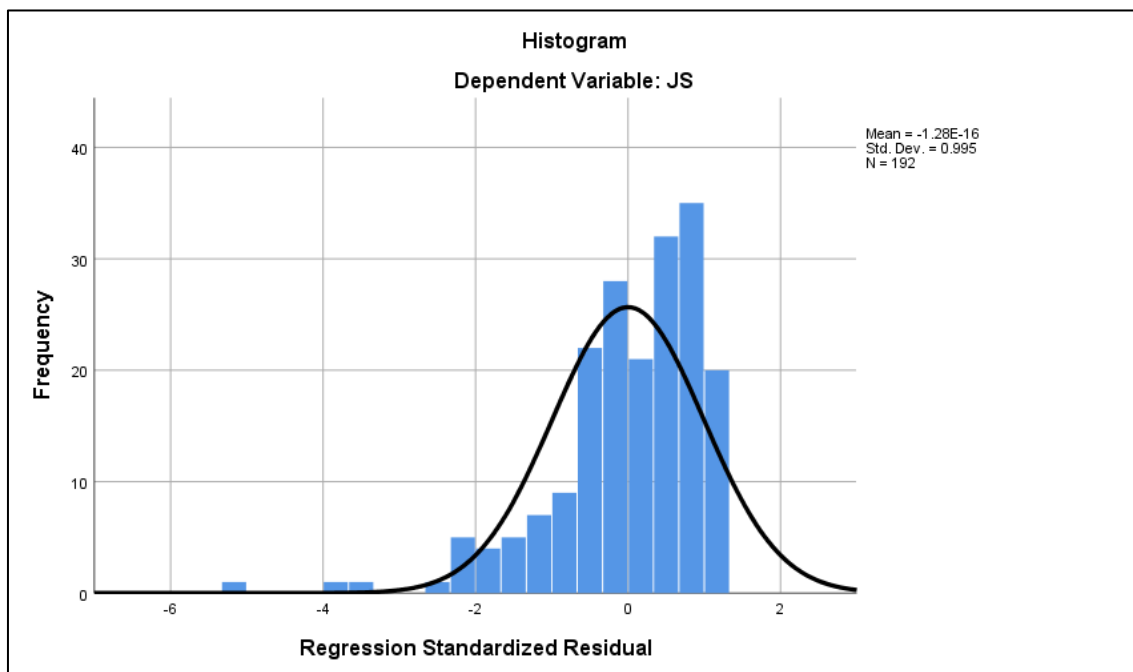
Figure 1: Normality Curve
