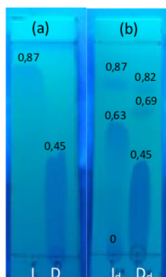
Fig. 6. TLC of ibuprofen and diclofenac before (I and D) and after ( I_d and D_d ) degradation
