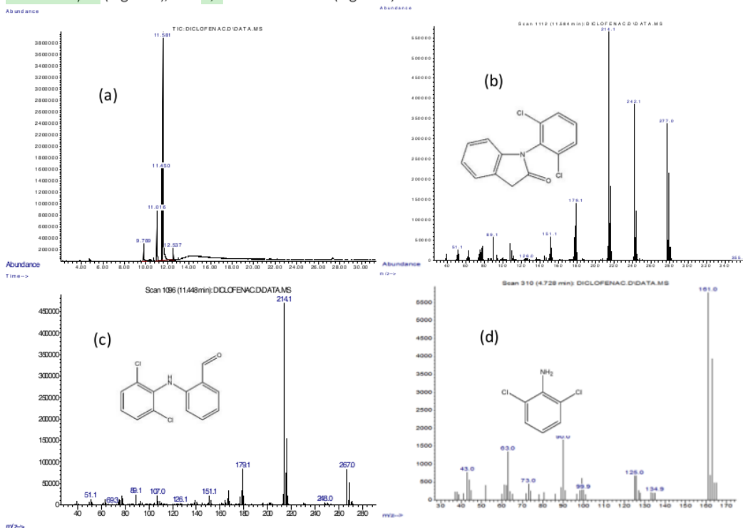
Fig. 10. Chromatogram diclofenac after degradation (a), MS diclofenac after degradation (b,c,d)
