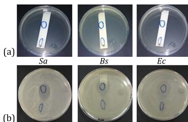
Figure 2. TLC-bioautographic of F extract of A. elegans SweF9 against S. aureus , B. subtilis , and E. coli . (a) before incubation; (b) after incubation
