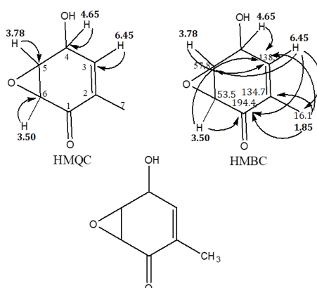
Figure 3. HMQC and HMBC correlation of compound 1 ((+)- epi -Epoformin)
