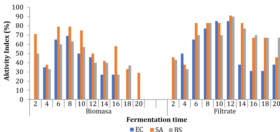
Figure 1. The index of antibacterial activity against the influence of fermentation time
