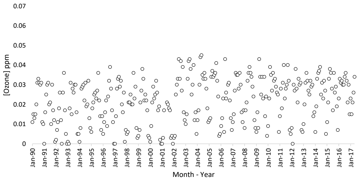
Figure 11: This is a plot of the minimum O 3 concentration for each month taken from the raw daily concentration values for sample site 06-037-0113, which is the station located in West LA.
