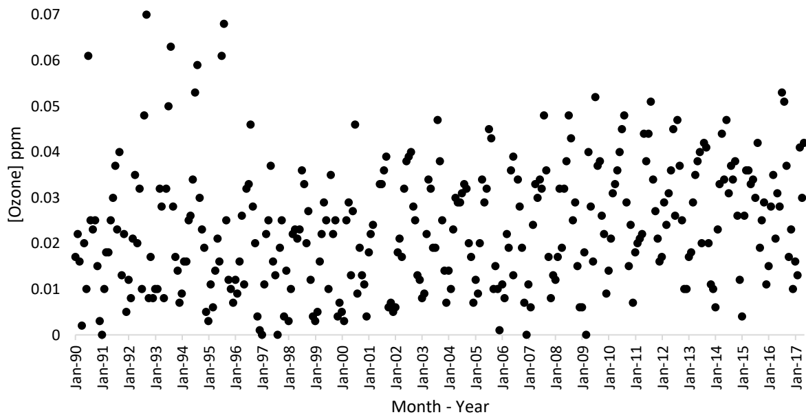
Figure 12: This is a plot of the minimum O 3 concentration for each month taken from the raw daily concentration values for sample site 06-037-0016, which is the station located in Glendora.
