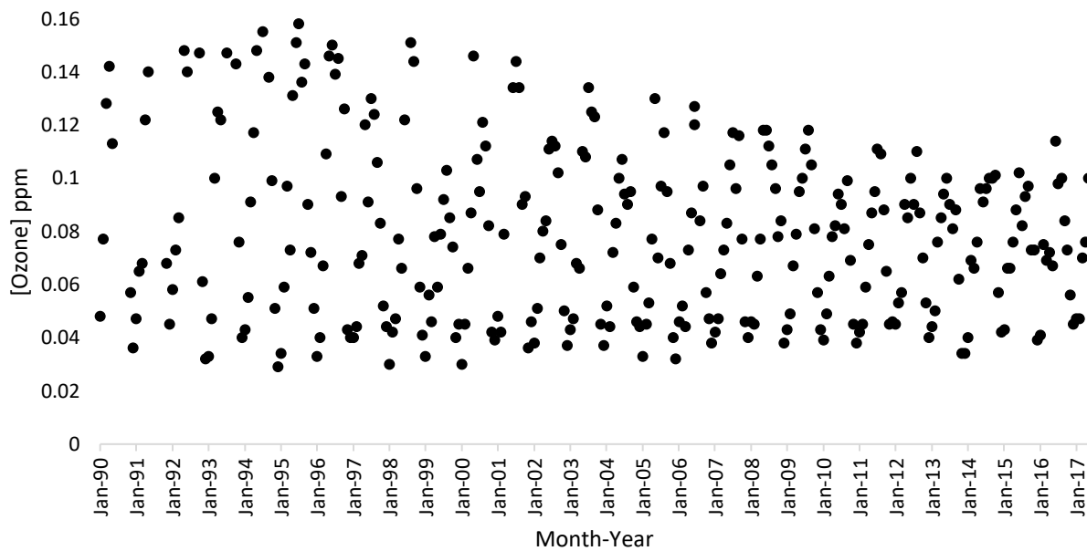
Figure 9: This is a plot of the maximum O 3 concentration for each month taken from the raw daily concentration values for sample site 06-037-0016, which is the station located in Glendora.
