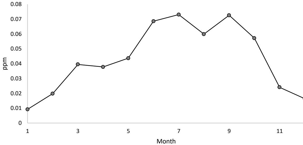
Figure 13: The plot of the monthly average values for the year 1990, with the months along the x-axis. The data is taken from sample site 06-037-1103. January is month 1, February is month 2, March is month 3, April is month 4, May is month 5, June is month 6, July is month 7, August is month 8, September is month 9, October is month 10, November is month 11, and December is month 12.
