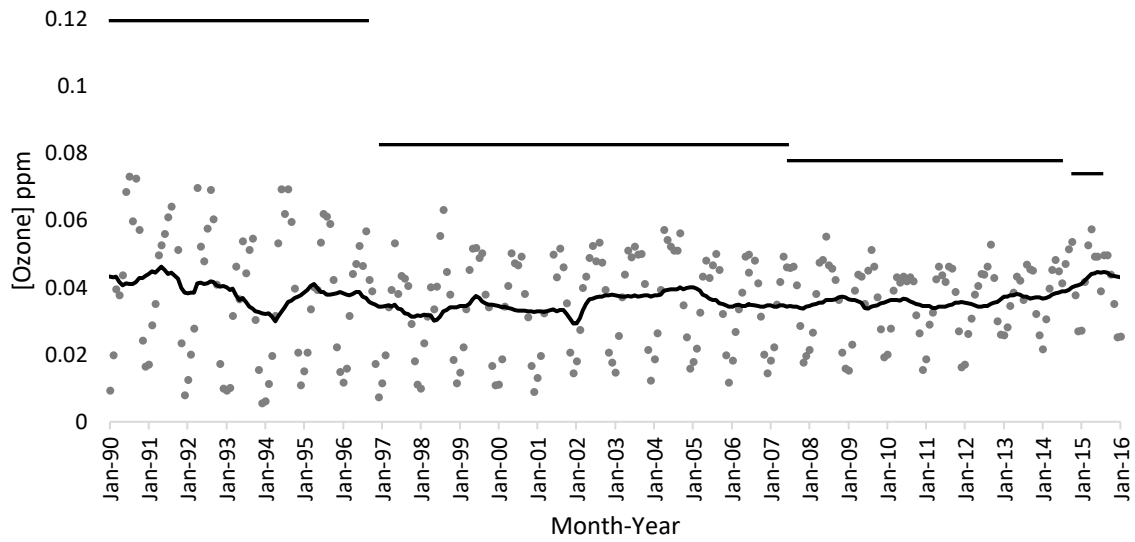
Figure 1: The plot of the monthly average O 3 concentration recorded by site ID 06-037-1103 from 1990 to the present, along with the running average of twelve data points.
