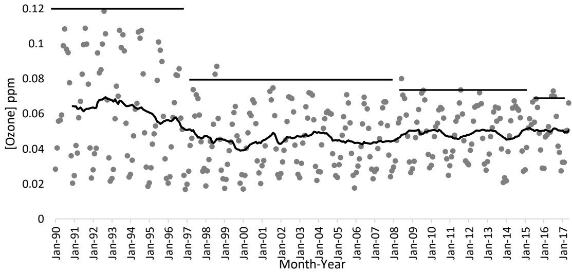
Figure 3: The plot of the monthly average O 3 concentration recorded by site ID 06-037-0016 from 1990 to the present, along with the running average of twelve data points.
