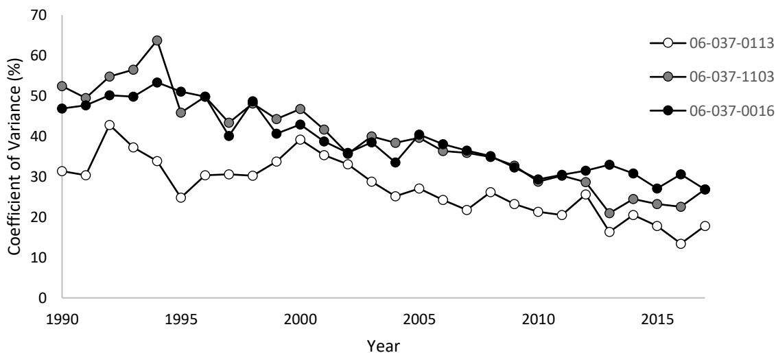
Figure 6: This is the plot of the annual coefficient of variance, recorded in a percentage value, for all three stations over the 27 year time span of the study.
