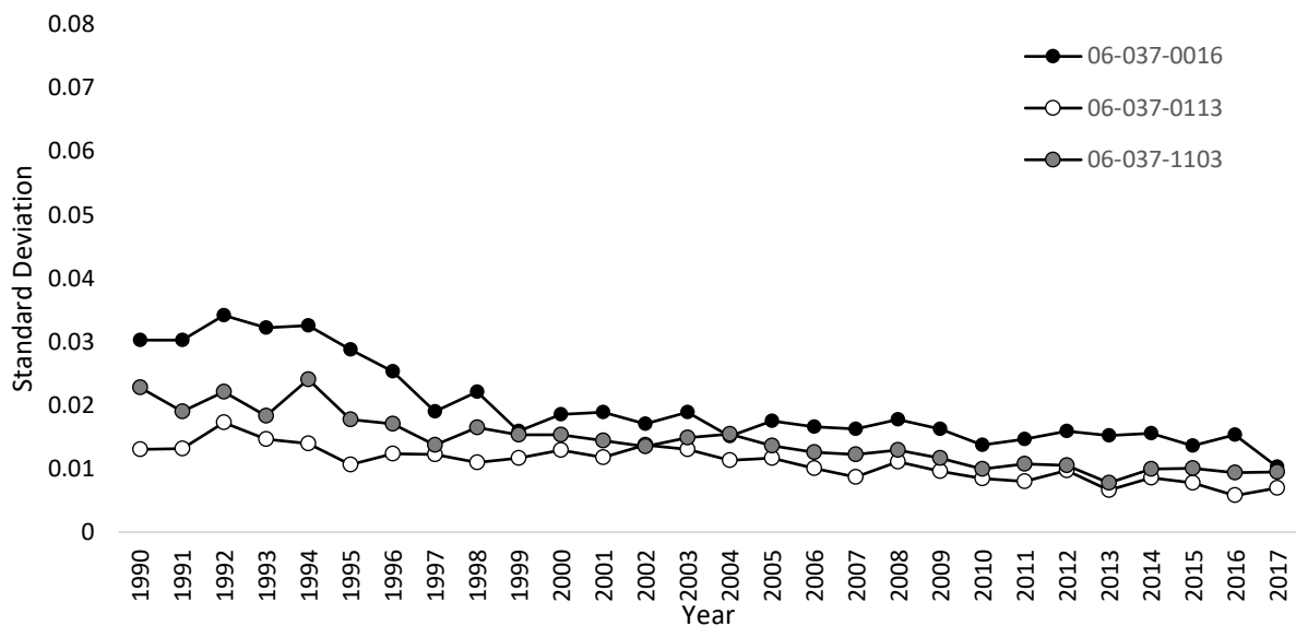
Figure 5: The standard deviation for the yearly averages graphed in Figure 4. These data points were calculated from the average monthly O 3 concentration values used to calculate each yearly average in Figure 4.
