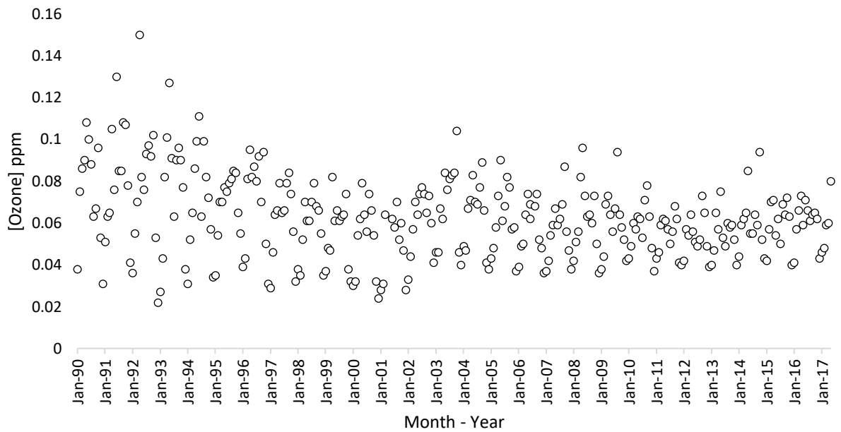
Figure 8: This is a plot of the maximum O 3 concentration for each month taken from the raw daily concentration values for sample site 06-037-0113, which is the station located in West LA.
