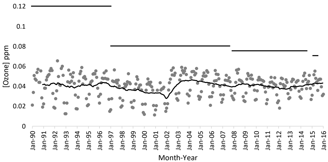
Figure 2: The plot of the monthly average O 3 concentration recorded by site ID 06-037-0113 from 1990 to the present, along with the running average of twelve data points.
