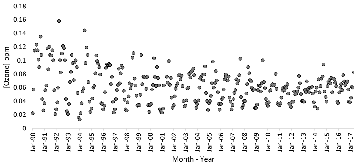
Figure 7: This is a plot of the maximum O 3 concentration for each month taken from the raw daily concentration values for sample site 06-037-1103, which is the station located on North Main Street, Downtown LA.
