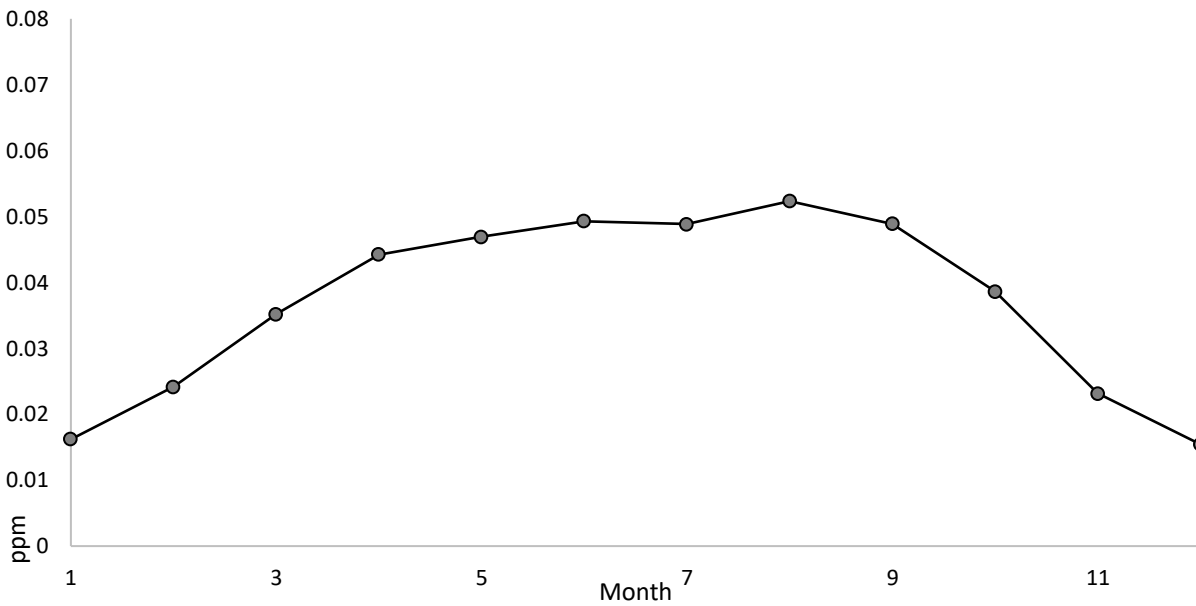
Figure 14: The plot of the monthly average values for the year 2016, the last full year in the study, with the months along the x-axis. The data is taken from sample site 06-037-1103. January is month 1, February is month 2, March is month 3, April is month 4, May is month 5, June is month 6, July is month 7, August is month 8, September is month 9, October is month 10, November is month 11, and December is month 12.
