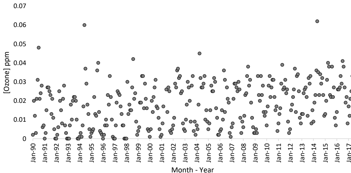
Figure 10: This is a plot of the minimum O 3 concentration for each month taken from the raw daily concentration values for sample site 06-037-1103, which is the station located on North Main Street, Downtown LA.
