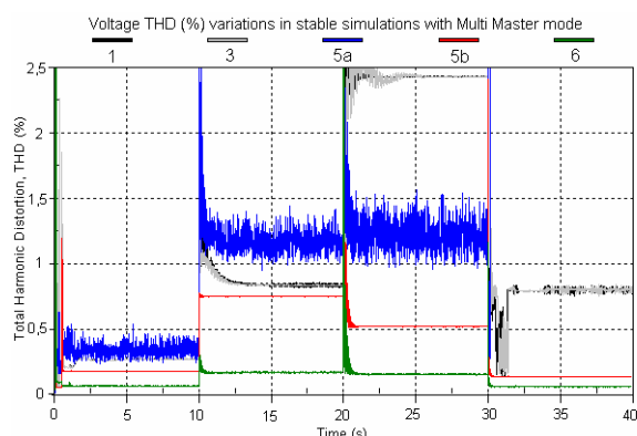
Figure 3. Voltage THD (%) variations during stable (table 5, 6, 7) simulations with Multi Master mode.
