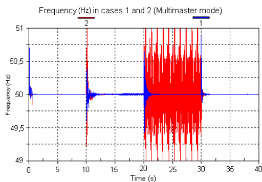
Figure 2. Frequency behaviour with Multi Master mode in cases 1 and 2.
