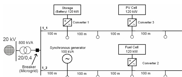
Figure 1. Studied urban LV network based microgrid.
