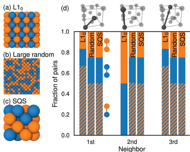
Figure 2. Alloys exhibit various degrees of order, spanning from ordered intermetallic phases such as a) L_{10} , to b) completely random. Order can be characterized by d) pair correlations, that is, the fraction of nearest neighbor pairs (1st, 2nd, 3rd, etc.) that are unlike (blue–orange) and alike (blue–blue and orange–orange). For example, 2/3 of the first nearest neighbor pairs in the L_{10} structure are blue–orange, while 1/3 are blue–blue or orange–orange. Large random structures at 50% concentration have 1/2 of its neighboring pairs (of any order) blue–orange, 1/4 blue–blue, and 1/4 orange–orange. The L_{10} structure can be represented by a unit cell with only two atoms, and is thus feasible to treat with LR-TDDFT. The large, random structure, on the other hand, is in general too large to be computed with LR-TDDFT. c) SQSs reproduce the pair correlations of large, random alloys using much smaller unit cells that are computationally tractable. SQSs are thus excellent models for random alloys in computationally relatively expensive methods such as LR-TDDFT.
