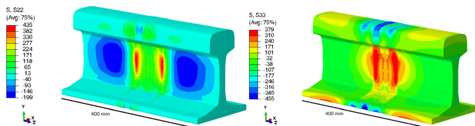
Fig. 13 Calculated residual stress (MPa) field after conventional ATW process with additional forging added (ALFONS module). S22 is vertical and S33 is longitudinal stress component
