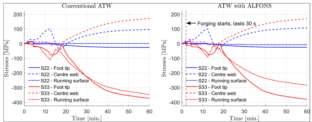
Fig. 10 Calculated development of stresses with time at weld center after pouring, forging starting 2 min (120 s) after pouring and ending at 2 min 30 s (150 s). Conventional ATW, left, and for the ATW process with additional forging (ALFONS module), right
