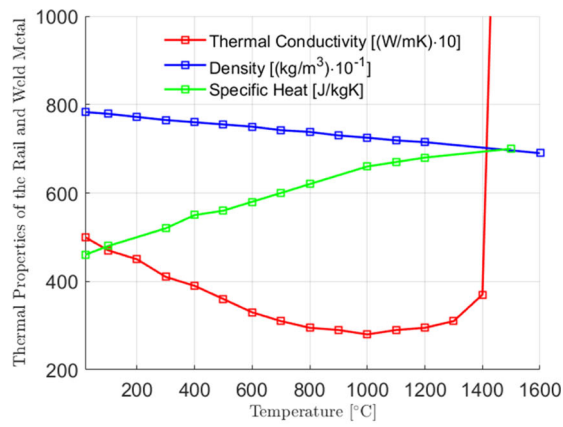
a Density, Conductivity and heat capacity variation with temperature estimated from Tuckova [22].
