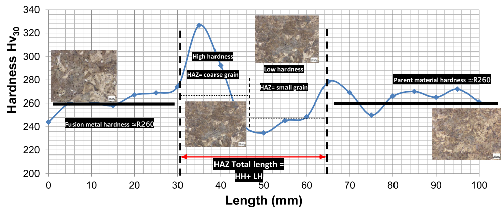
Fig. 19 Relationship between the metallurgical gradient and the hardness variation across a thermite weld
