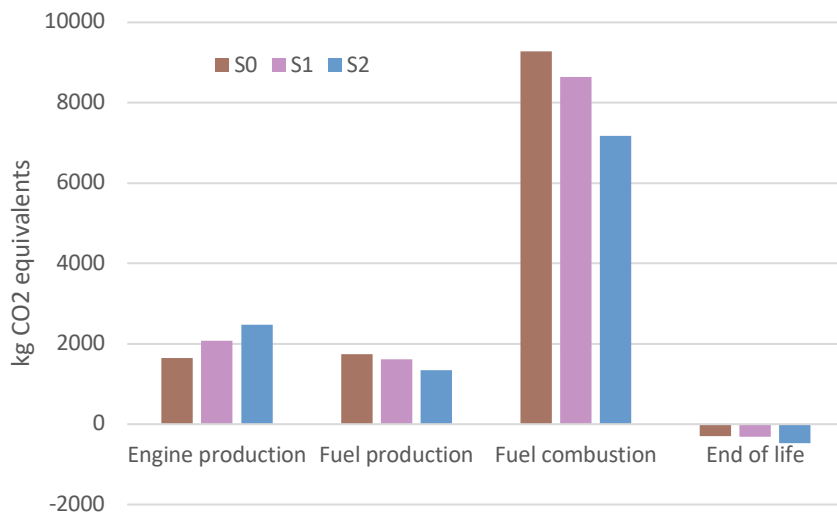
Figure 11. Emissions of greenhouse gases for the different life cycle stages of the engine, as represented by kg CO 2 -equivalents per functional unit for each scenario S0, S1 and S2, from Böckin and Tillman (2019). The total reduction of greenhouse gas emissions compared to S0 is 3 % for S1 and 15 % for S2.
