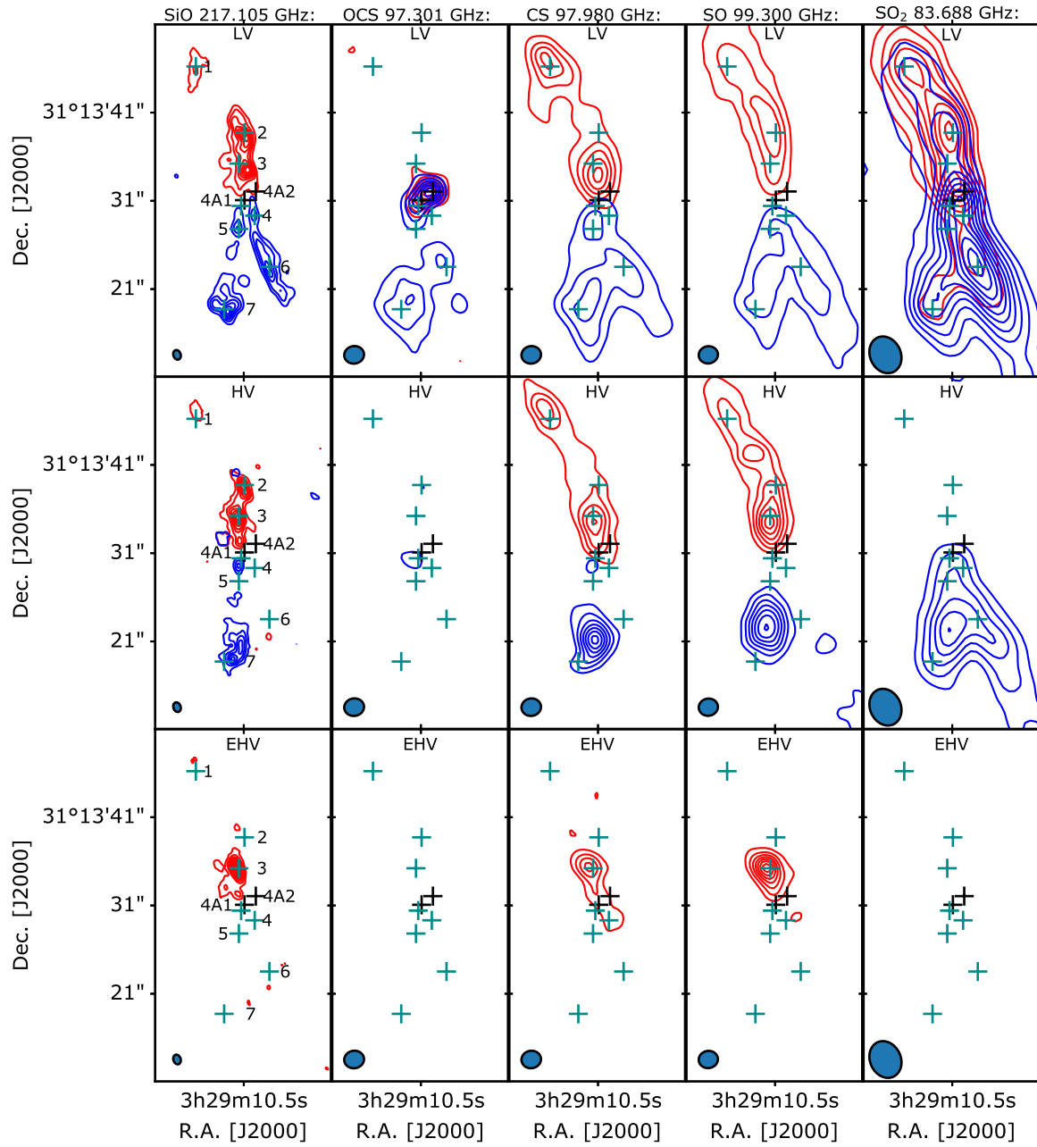
Fig. A.1. Channel maps of the main sulfuretted isotopologues observed at low ( \sim 2-4'' ) resolution for three velocity ranges: low-velocity LV ( -10, +5 ) and ( +10, +25 ) km s -1 , high-velocity HV ( -20, -11 ) and ( +26, +40 ) km s -1 , and extremely-high-velocity EHV ( -35, -21 ) and ( +41, +55 ) km s -1 .
