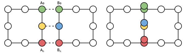
Figure 2: Left. A seam is defined between two patches. Right. Distance constraints with zero rest length bring the particles together.
