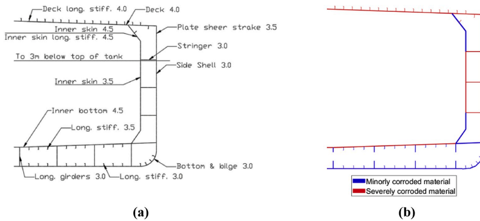
Fig. 4. (a) Corrosion margins (unit: mm) and (b) different material models used for the corroded ship cases T5I and T5D.
