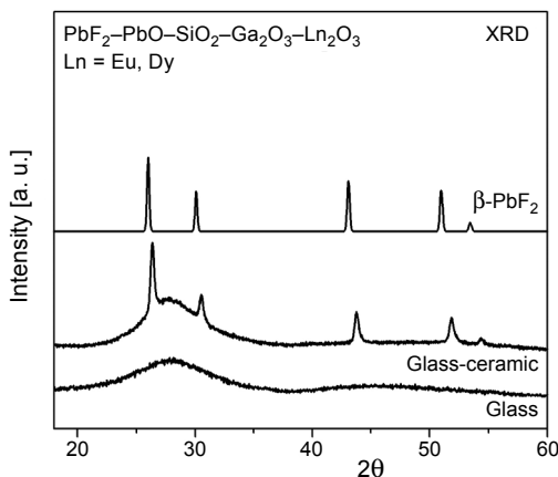
Fig. 2. X-ray diffraction pattern for the \text{PbF}_2\text{--PbO--SiO}_2\text{--Ga}_2\text{O}_3\text{--Ln}_2\text{O}_3 glass (Ln = Eu or Dy) before and after heat treatment.
