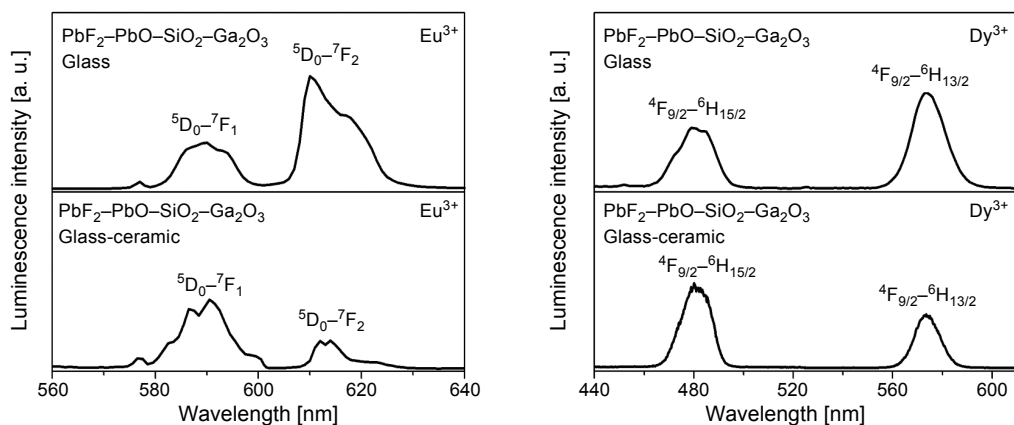
Fig. 3. Luminescence spectra for Eu 3+ (left) and Dy 3+ (right) ions in the heavy metal oxyfluoride lead silicate glass systems before and after heat treatment.
