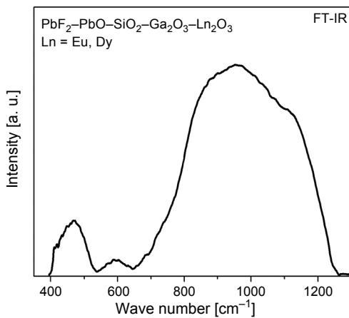
Fig. 1. FT-IR spectrum for the \text{PbF}_2\text{--PbO--SiO}_2\text{--Ga}_2\text{O}_3\text{--Ln}_2\text{O}_3 glass (Ln = Eu or Dy).
