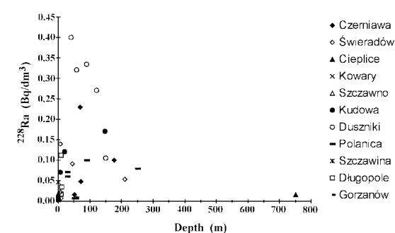
Fig. 5. The correlation between ^{226}\text{Ra} and ^{228}\text{Ra} concentrations and the depth of water extraction for 55 groundwater springs and intakes in the Polish part of the Sudety Mts.
