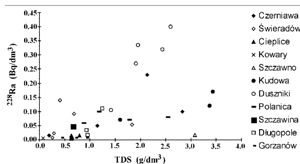
Fig. 4. The correlation between ^{226}\text{Ra} and ^{228}\text{Ra} concentrations and the TDS value of water for 55 groundwater springs and intakes in the Polish part of the Sudety Mts.
