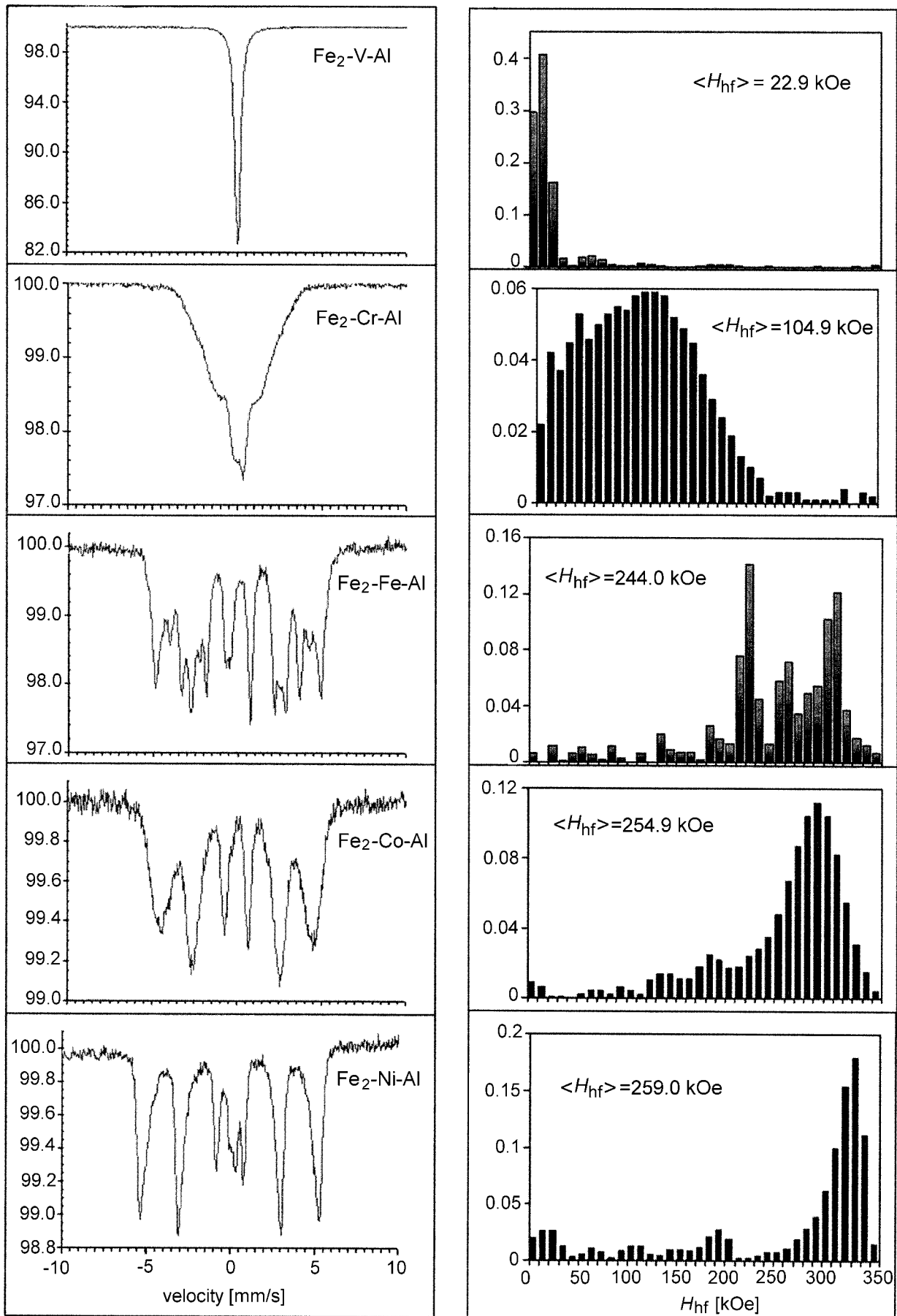
Fig. 4. Mössbauer spectra and hyperfine field distributions for the \text{Fe}_2\text{MAl} with \text{M} = \text{V}, \text{Cr}, \text{Fe}, \text{Co} and \text{Ni} .
