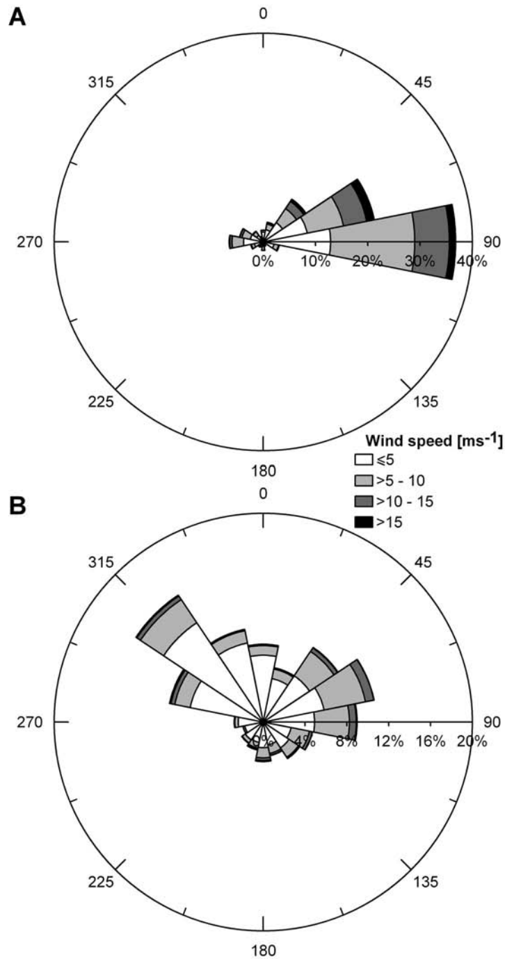
Fig. 5. The distribution of wind directions and wind speed at Hornsund in winter seasons (OCT-MAY) 1978-2011 (A), and at Hansbreen in winter seasons 2007/2011 (B). Locations shown on Fig. 2A at PPS and AWS, respectively.
