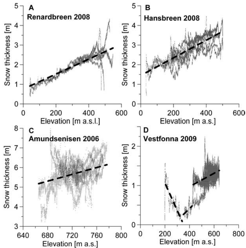
Fig. 10. Relations of snow thickness to altitude on the studied glaciers.
