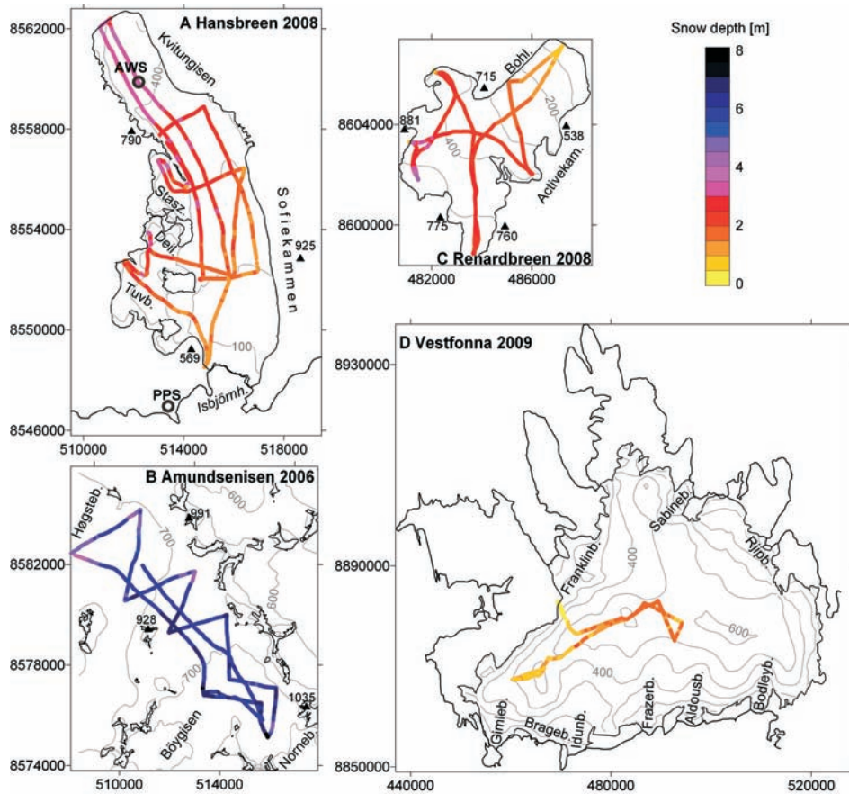
Fig. 2. Snow thickness on glaciers investigated by GPR during 2006–2009. The coordinate system of maps A–C is UTM 33X on WGS84. Map scale for Vestfonna (D) is smaller than for the other glaciers. Vestfonna is located on the border between UTM zones 33X and 35X. To use homogenous coordinates for the entire map (D) we adopted UTM coordinates for the non-standard zone 34X, which is not applied in cartographical works. PPS – Polish Polar Station in Hornsund, AWS – automatic weather station in Hansbreen accumulation zone, Tuvb. – Tuvbreen, Deil. – Deileggbreen, Stasz. – Staszelisen, Isbjørnh. – Isbjørnhamna, Høgsteb. – Høgstebreen, Norneb. – Nornebreen, Bohl. – Bohlinryggen, Activekam. – Activekammen, Franklinb. – Franklinbreane, Sabineb. – Sabinebreen, Rjipb. – Rjipbreen, Bodleyb. – Bodleybreen, Aldousb. – Aldousbreen, Frazerb. – Frazerbreen, Idunb. – Idunbreen, Brageb. – Bragebreen, Gimleb. – Gimlebreen.
