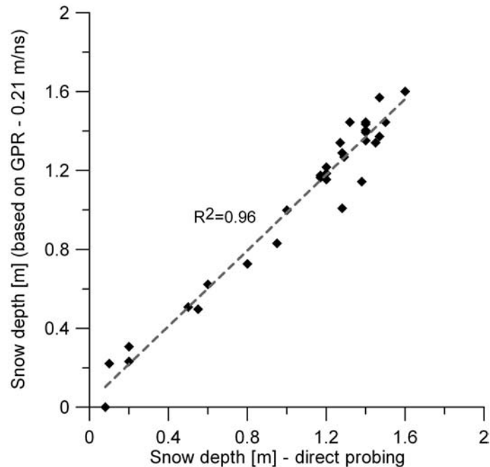
Fig. 6. Comparison of results of snow thickness measurements based on GPR soundings with those of classical probing, Vestfonna 2009.
