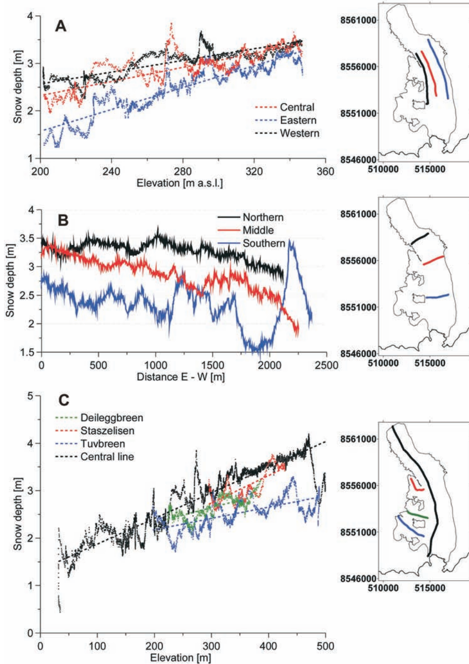
Fig. 8. GPR derived snow thickness and relations to altitude and distance on Hansbreen in April 2008 measured in particular profiles: A – parallel profiles: eastern, central and western in elevation range 200–350 m a.s.l., B – southern, middle and northern profiles, C – profiles along the central line and along tributary glaciers.
