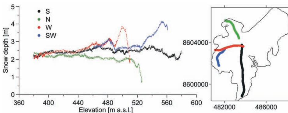
Fig. 7. Relations of snow thickness to altitude recorded in particular profiles above 370 m a.s.l. on Renardbreen in April 2008.
