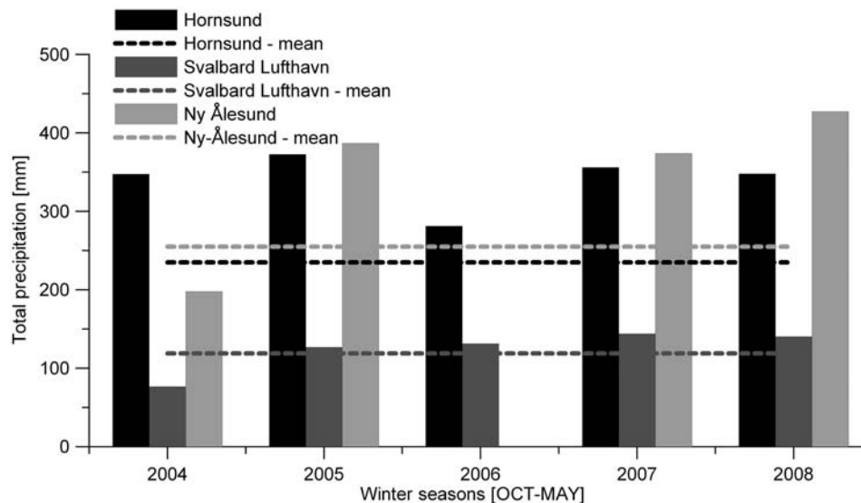
Fig. 4. Total precipitation in winter seasons (OCT-MAY) 2004/2005–2008/2009 and mean long-term sum of precipitation in winter season recorded at Svalbard meteorological stations .
