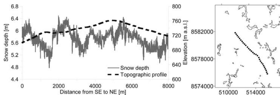
Fig. 9. Variability of snow thickness and elevation changes along the axis of Amundsenisen (April 2006).
