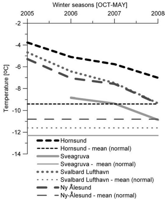
Fig. 3. Mean temperatures of winter seasons (OCT-MAY) 2005/2006–2008/2009, and long-term average winter temperatures over the normal period (1961–1990), at Svalbard meteorological stations.
