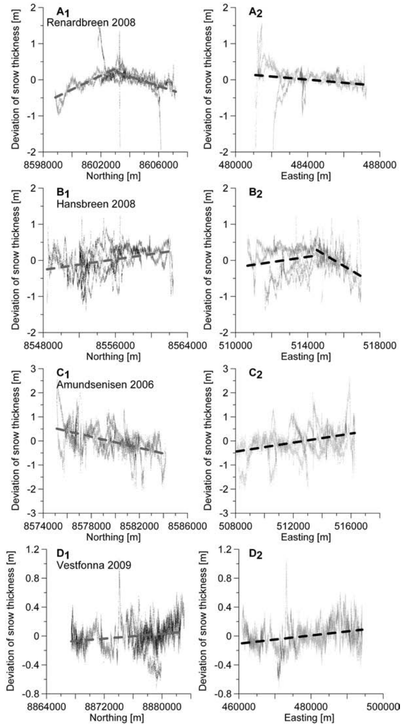
Fig. 11. Normalized directional gradients of snow accumulation (S-N in left column; W-E in right column). Coordinate systems: UTM 33X on wgs84 (A–C), and non-standard UTM 34X on wgs84 (D).
