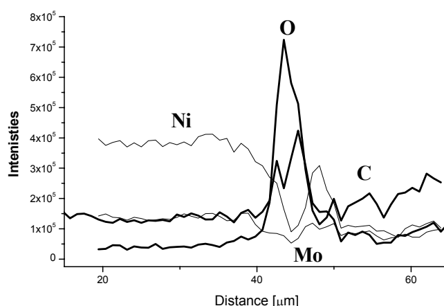
Fig. 5. Scan lines of the experimental intensities of the main Auger lines for elements Ni, O, Mo, and C obtained for Ni-Mo layers with polyethylene (Ni-Mo+PE) – 50 mA/cm 2 .
