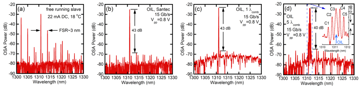
Fig. 3. Spectra of the same slave microring laser with (a) free-running state, and locked by (b) Santec master laser, (c) single-comb line (1λ) and (d) one wavelength (C3) out of five-comb lines (5λ). (inset: zoom-in spectra of filtered 5 comb lines with C3 line locking the slave).
