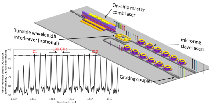
Fig.1. Schematic of a proposed fully heterogeneously integrated OIL DWDM system-on-chip. Inset: measured spectrum of a heterogeneous QD comb laser demonstrated recently [4].
