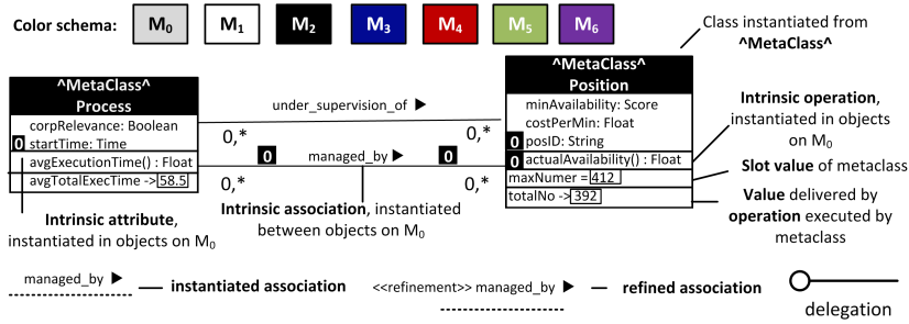
Fig. 1: Concrete Syntax of FMML x [15]
