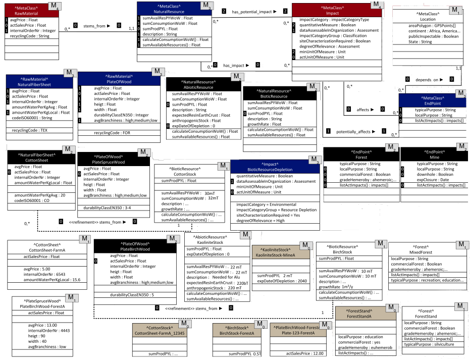
Fig. 2: An excerpt from the LCA multi-level model
