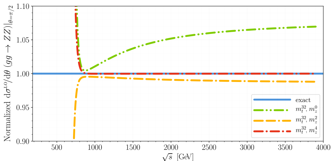
Figure 4. LO partonic differential cross section for gg \rightarrow ZZ for \theta = \pi/2 , normalized to the exact result. The three high-energy expansions contain terms up to order m_t^{32} and m_Z^0 , m_Z^2 and m_Z^4 .
