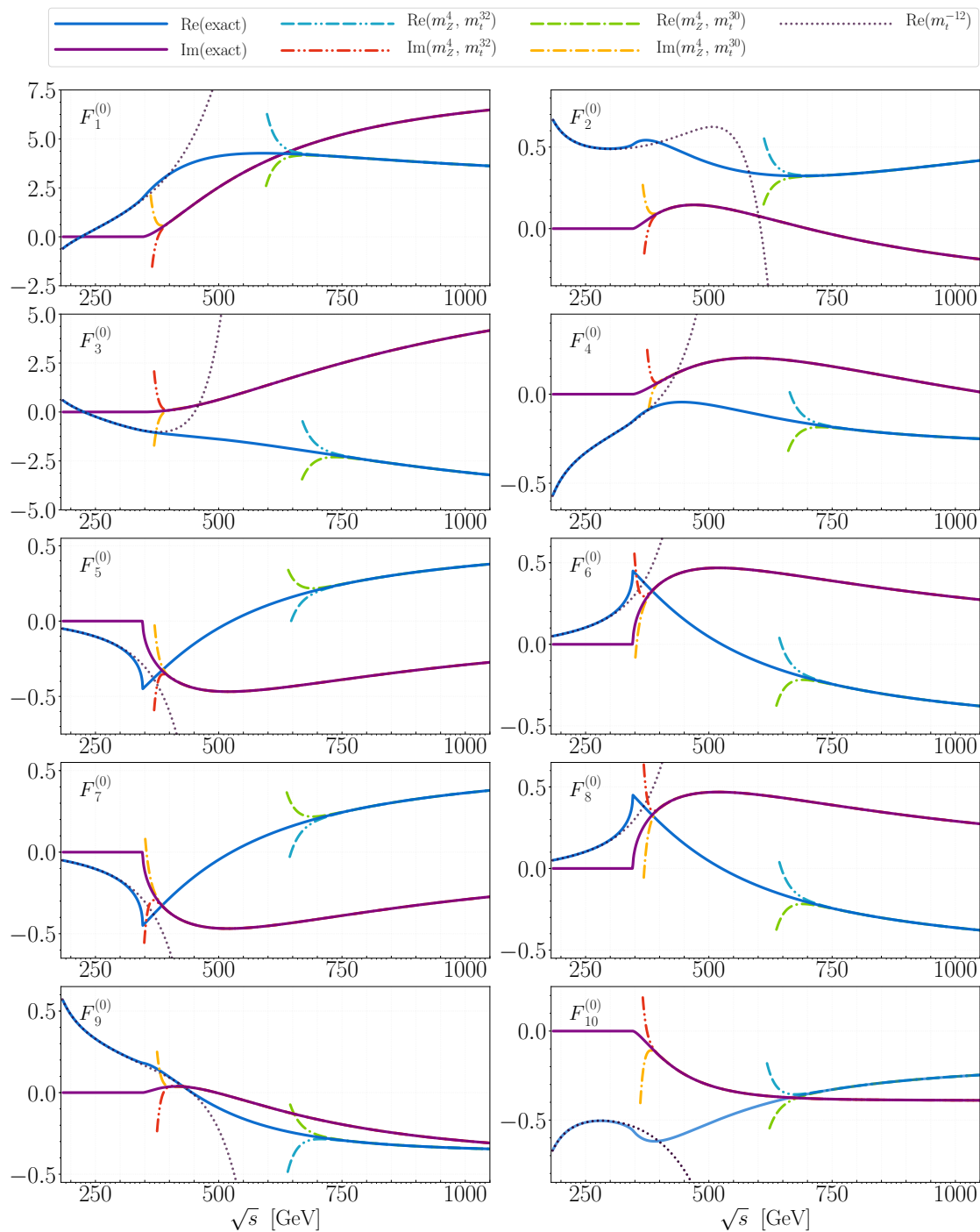
Figure 9. F_1^{(0)}, \dots, F_{10}^{(0)} as a function of \sqrt{s} , for \theta = \pi/2 .
