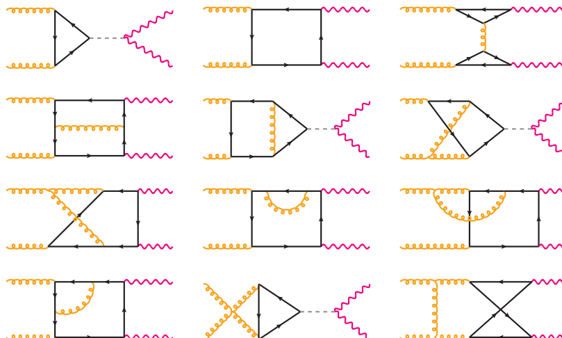
Figure 1. Sample LO and NLO Feynman diagrams for gg \rightarrow ZZ . “Double triangle” diagrams (such as the third diagram) are known, and not considered here.
