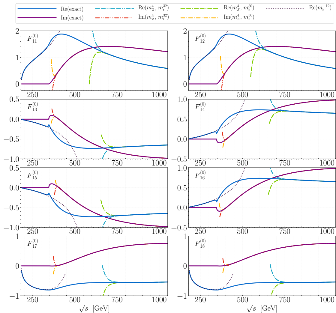
Figure 10. F_{11}^{(0)}, \dots, F_{18}^{(0)} as a function of \sqrt{s} , for \theta = \pi/2 .
