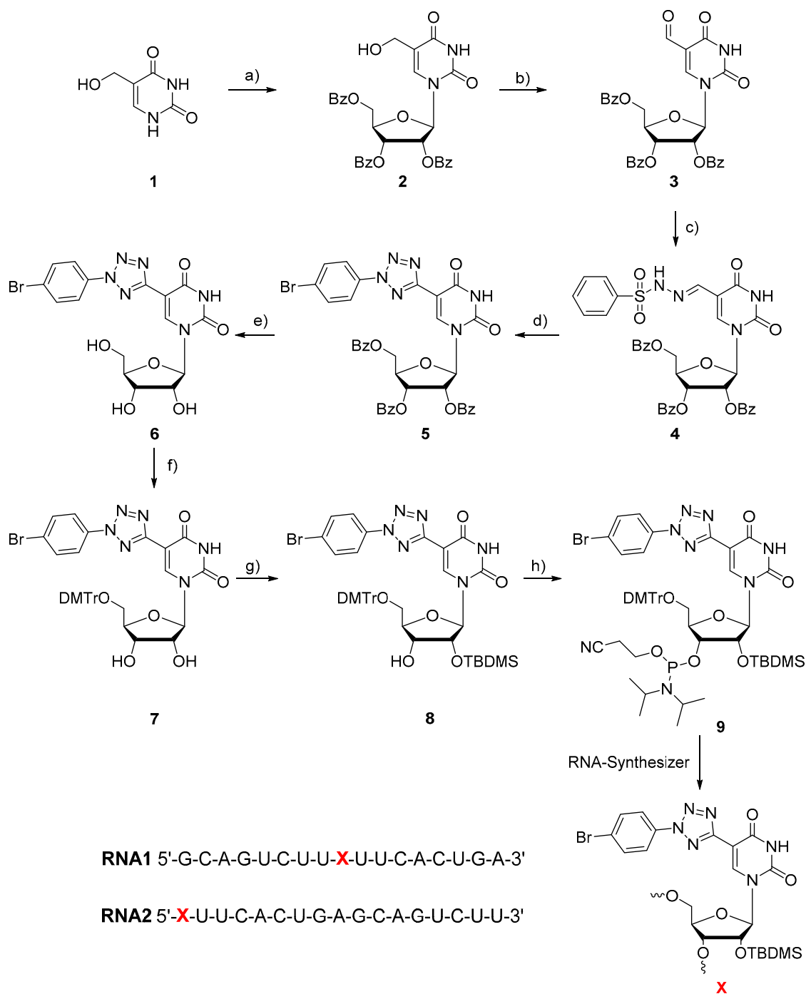
Scheme 1. Synthesis of RNA building block 9: (a) 2,3,5-Tribenzoyl- \beta -D-ribofuranoside-1-acetate, N,O-bis(trimethylsilyl)acetamide, trimethylsilyl trifluoromethanesulfonate, acetone, 60 °C, 2 h, 70%. (b) Dess-Martin periodinane, \text{CH}_2\text{Cl}_2 , r.t., 2 h, 72%. (c) Benzenesulfonyl hydrazide, dichloromethane, 40 °C, 2 h, 82%. (d) 4-bromobenzene diazonium tetrafluoroborate, pyridine, -15 °C, 0.5 h, 48%. (e) Ammonia (7M) in MeOH, 80 °C, 24 h, 65%. (f) DMT-Cl, silver(II) nitrate, pyridine, r.t., 2 h, 61%. (g) \text{AgNO}_3 , TBDMS-Cl, pyridine, r.t., 6 h, 36%. (h) DIPEA, 2-cyanoethyl N,N -diisopropyl-chlorophosphoramidite, \text{CH}_2\text{Cl}_2 , r. t., 6 h, 87%.
