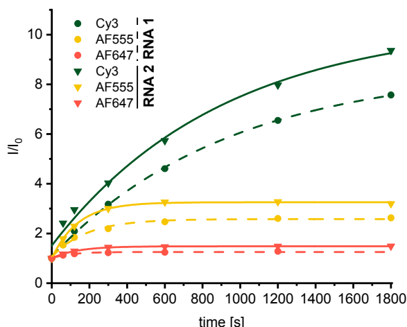
Figure 3. Fluorescence intensity changes during the photoclick modification of RNA1 (2.5 \mu\text{M} , dashed lines) and RNA2 (2.5 \mu\text{M} , solid lines) in the presence of Cy3-maleimide, AF555-maleimide and AF647 maleimide (each 3.75 \mu\text{M} , 1.5 equiv.); irradiation at 300 nm, fluorescence excitation at 358 nm, in 10 mM Na-P i buffer (250 mM NaCl, pH 7). I_0 is the fluorescence intensity before the irradiation.
