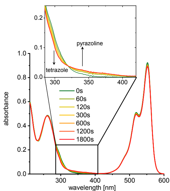
Figure 2. UV/Vis absorbances recorded during irradiation of RNA1 (2.5 \mu\text{M} ) with 1.50 equiv. AF555-maleimide (3.75 \mu\text{M} ) in 10 mM Na-P i buffer (250 mM NaCl, pH 7).
