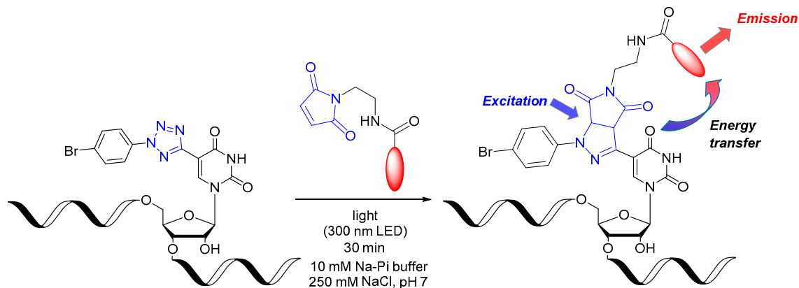
Figure 1. Principle of fluorogenic RNA photoclick labeling using the tetrazole-modified uridine (marked in blue, for building block structure see Scheme 1) as a photoreactive building block in single-stranded RNA and maleimide-conjugated dyes (maleimide marked in blue, dye in red). The energy transfer between the pyrazoline as a photoclick product and the attached dye yield a fluorogenic photoclick reaction.
