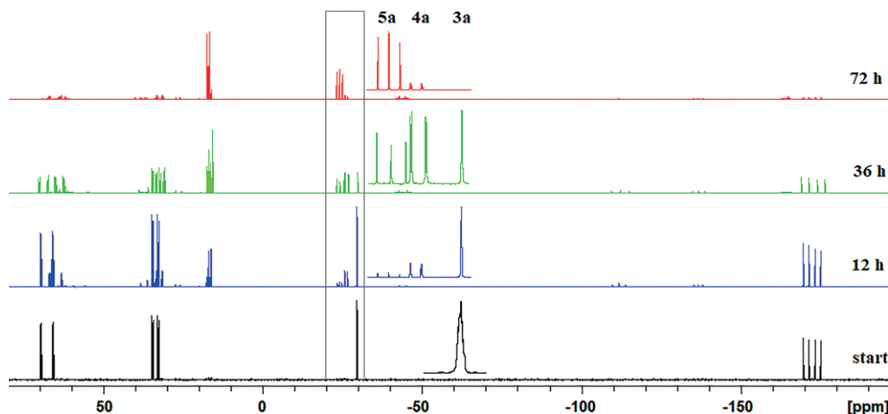
Figure 1. ^{31}\text{P}\{^1\text{H}\} NMR spectra of the decomposition of 3a in \text{C}_6\text{D}_6 at 25^\circ\text{C} . Bottom trace: pure 3a ; second trace: decomposition beginning ( \mathbf{3a} > \mathbf{4a} > \mathbf{5a} ); third trace: further decomposition; top trace: \mathbf{5a} \gg \mathbf{4a} , no 3a remains.
