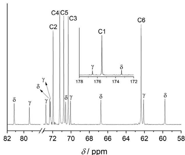
Fig. 4. 13 C NMR spectra of HGluc (C1–C6) and its \gamma - and \delta -lactones. Experimental conditions: t = 25^\circ\text{C} , I = 0.8\text{ M} (NaCl), 20 %V/V D 2 O; [\text{NaGluc}]_{\text{T}} = 0.320\text{ M} , [\text{HCl}]_{\text{T}} = 0.369\text{ M} . The figure has been replotted based on the data of Ref. [82].
