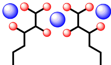
Fig. 16. Schematic structure of the short-chain polynuclear complex built up of \text{Ca}^{2+} ions (blue circles) and \text{GlucH}_2^{\ominus 2} ions (the coordinating oxygens of which are represented by red circles).
