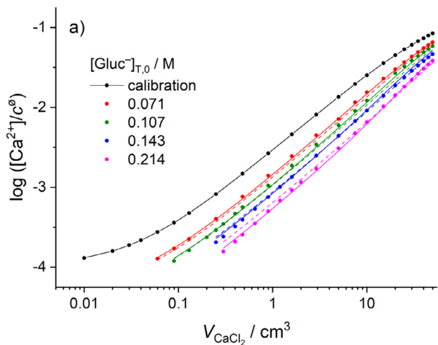
Fig. 5. \text{Ca-ISE} titration curves in the \text{Ca(II)}/\text{Gluc}^- system; y axis: logarithm of the concentration of free \text{Ca}^{2+} , x axis: added volume of the titrant \text{CaCl}_2 . Experimental conditions: t = (25.0 \pm 0.1)^\circ\text{C} , I = 1\text{ M (NaCl)} , V_0 = 70\text{ cm}^3 ; [\text{CaCl}_2]_{\text{T},0} = 10^{-4}\text{ M} . The initial total concentrations of the ligand are shown in the legend. The concentration of the titrant \text{CaCl}_2 was 0.201\text{ M} . Symbols refer to the measured data; lines were calculated by assuming the formation of the \text{CaGluc}^+ complex (dashed), or both the \text{CaGluc}^+ and \text{CaGluc}_2^0 complexes (solid). The figure has been replotted based on the data of Ref. [70].
