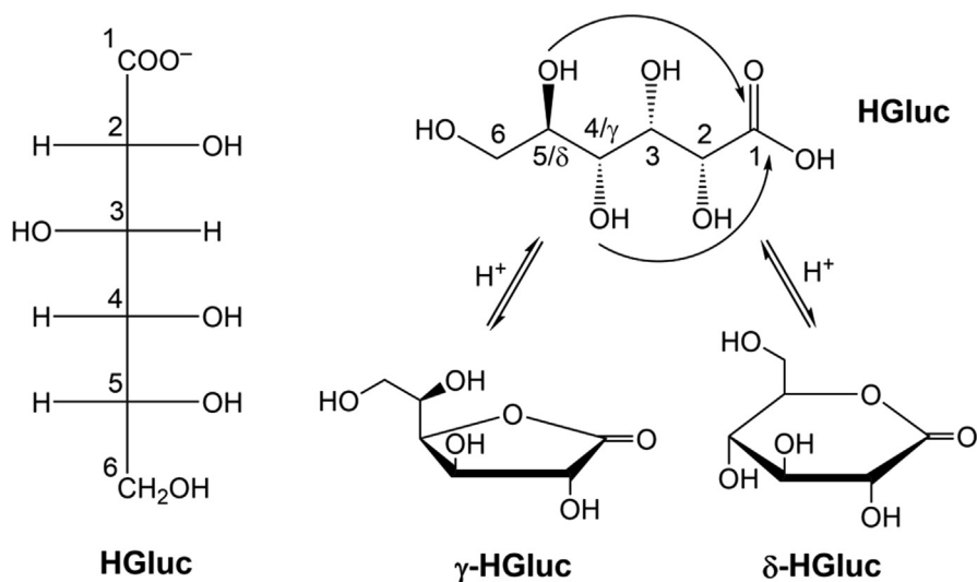
Scheme 1. Chemical formula of D-gluconic acid (HGluc), as well its five- ( \gamma -HGluc) and six-membered ( \delta -HGluc) lactones. Additionally, the nucleophilic attack of the OH group being the initial step in the acid-catalyzed lactonization is indicated.
