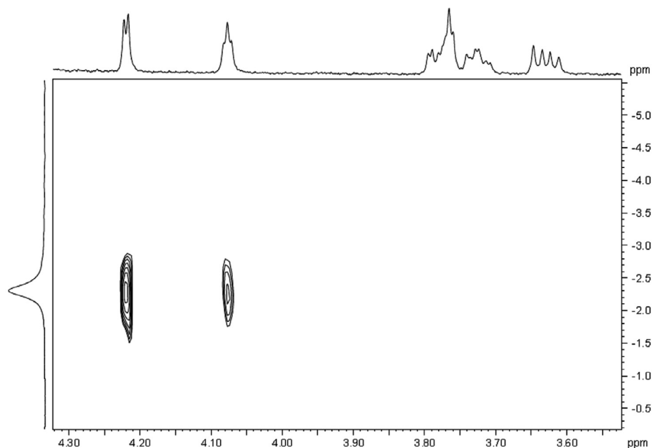
Fig. 8. The 2D ^1\text{H} - ^{43}\text{Ca} HMQC spectrum ( ^1\text{H} : x, ^{43}\text{Ca} : y axis) of the solution containing 0.2 M \text{CaCl}_2 and 0.2 M \text{NaGluc} . The peaks of H(C2) and H(C3) are seen around 4.24 and 4.08 ppm, respectively. Reproduced with permission [25] Copyright 2010 Elsevier.
