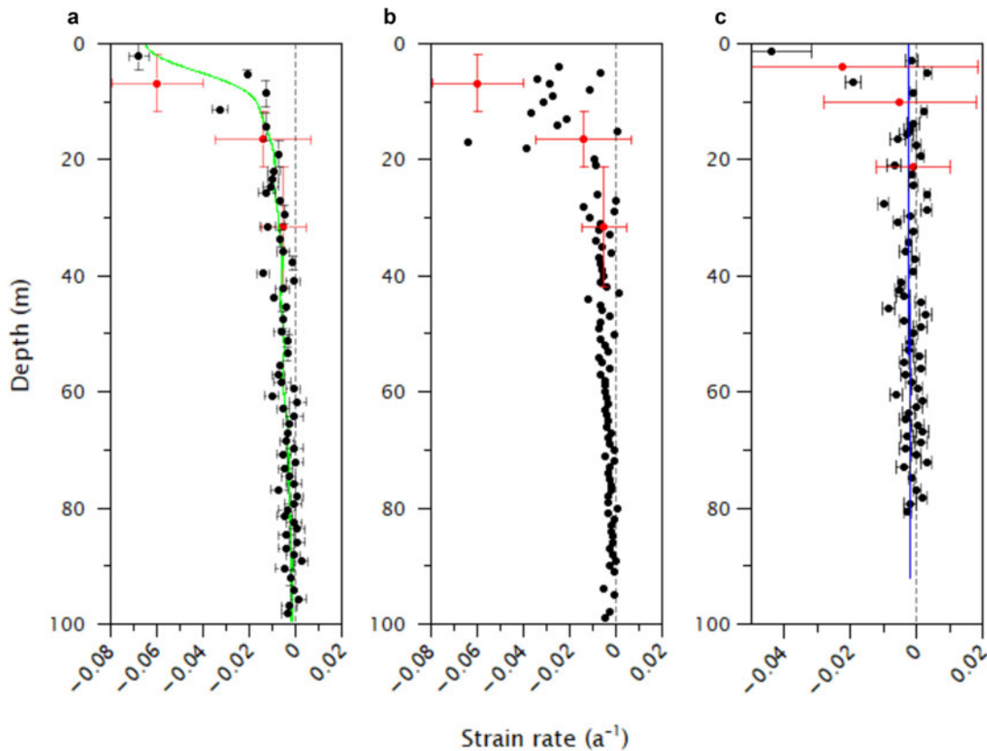
Fig. 5. Vertical strain rates at IC12 (a) measured between 60 OPTV markers as raw data (black dots) and following regularisation (green line), and by three CCM experiments (red dots), (b) similar to (a) but calculated by the XCM following luminosity trace shifting, and (c) as ice-equivalent vertical strain to allow comparison with modelled strain rates (blue line). Horizontal bars represent strain-rate uncertainty (see text) and the vertical bars represent the depth range over which discretised strain is calculated. Note the uncertainty presented for ice-equivalent vertical strain in (c) omits (unconstrained) uncertainty in density; the actual uncertainty range in (c) is therefore greater than illustrated.
