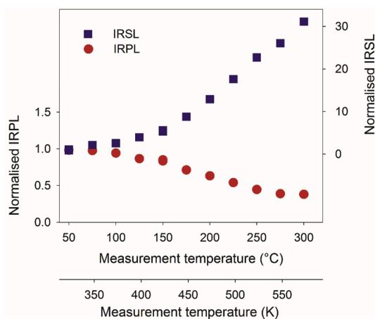
Fig. 6. Change in IRPL and IRSL signals with measurement temperature. Note the different y-axes used for the IRPL and IRSL data. The temperature is shown both in centigrade and kelvin to allow comparison with previously published data.
