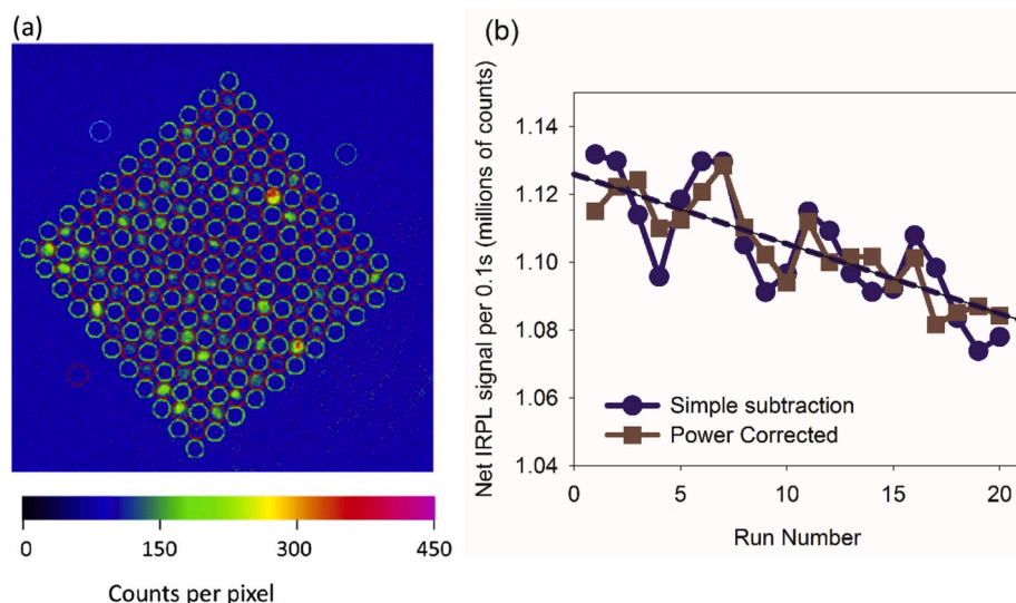
Fig. 4. (a) Regions of interest defined both to estimate the IRPL signal (shown as red circles) and to define the background due to breakthrough (shown as green circles). (b) Net IRPL signal for the holes with sample (red circles in part a). Each run involved 2.5 s of stimulation at 850 nm, but data are expressed as signal per 0.1s. (For interpretation of the references to colour in this figure legend, the reader is referred to the Web version of this article.)
