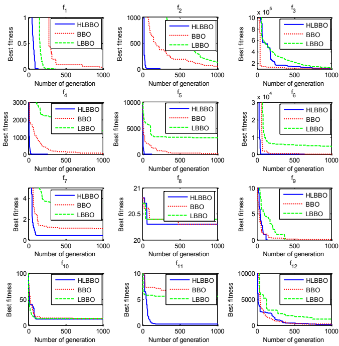
Fig. 2. Converge curves of the HLBBO, BBO and LBBO algorithms on test functions f_1 - f_{12} .
