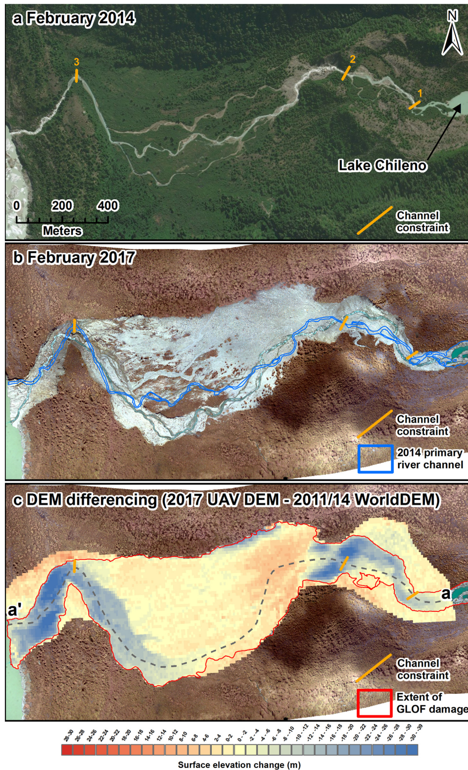
Fig. 4. Geomorphology of the Chileno Valley before (a) and after (b) the GLOF event that occurred in December 2015. Post-GLOF surface elevation changes are shown in image (c).
