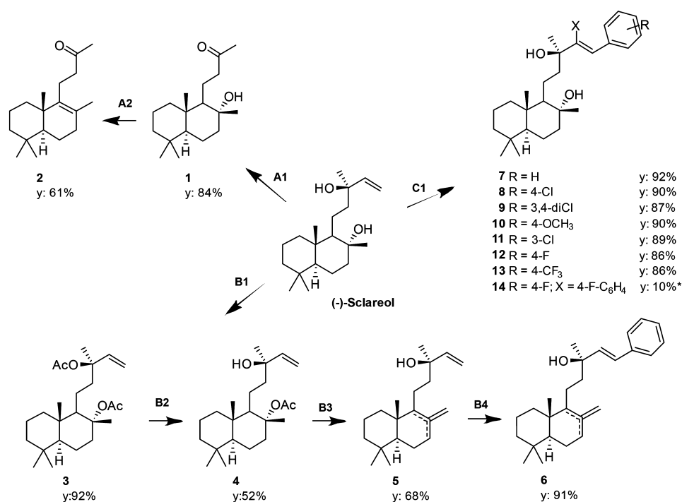
A1: KMnO 4 / MgSO 4 / acetone / rt / overnight A2: I 2 / toluene / reflux / 3 h B1: AcCl / N,N-DMA / DCM / rt / 24 h B2: KOH / H 2 O / EtOH / rt / 24 h B3: NaHCO 3 / DMSO / 100 W / 200 °C / 11 min (microwave-assisted) B4 = C1: Ar-B(OH) 2 / Pd(OAc) 2 / Cu(OAc) 2 / NaOAc / DMF / 130 °C / 300 W / 12 min (microwave-assisted; *classic thermal for 14 at 80 °C, 6 h). y = yield.
