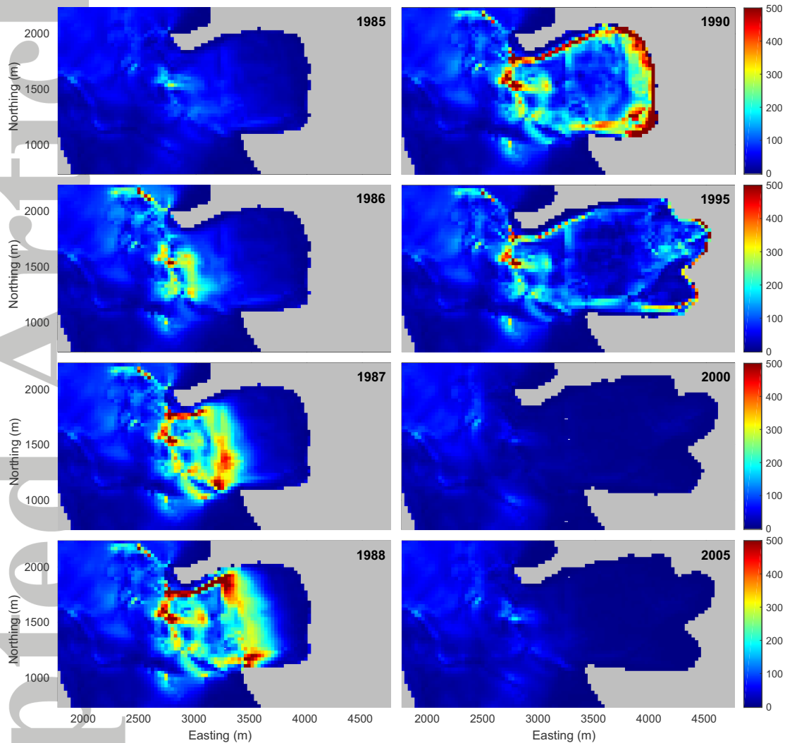
Figure 13. Maps of the vertically-integrated deformational power density at various times in the surge cycle. The 1985 snapshot corresponds to the surge onset; 1986, 1987, 1988 correspond to the 3-year accelerating phase of the surge; 1990 and 1995 to the continuing surge. The 2-year decelerating phase from 1996–1998 is not shown; post-surge snapshots for 2000 and 2005 complete the cycle.
