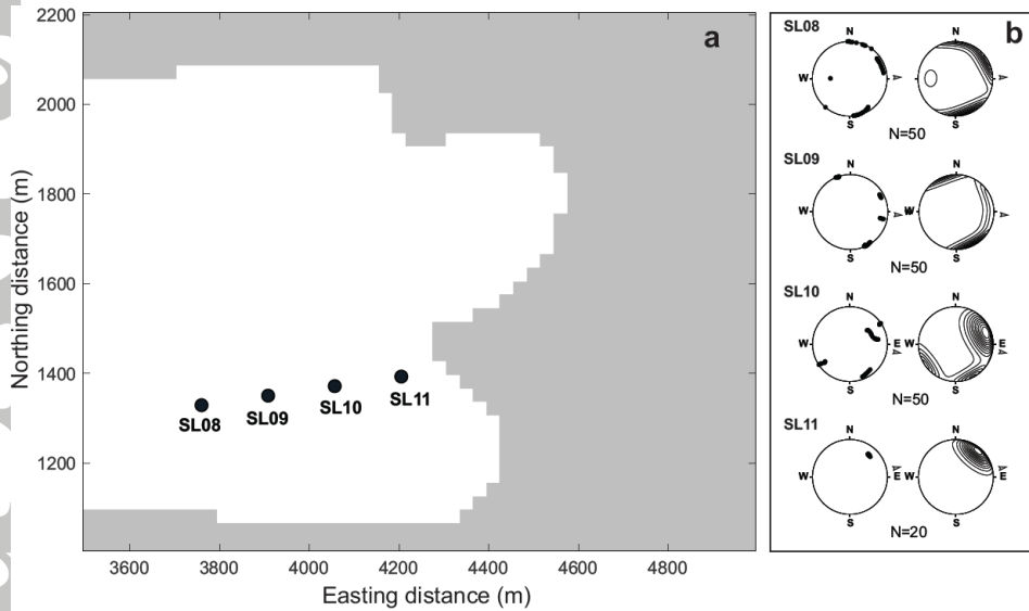
Figure 22. Simulated orientation of surface cracks at centerline sites (but not field measurement sites) near the terminus of Trapridge Glacier. Observation year is 2006.6 (year 21.6 of the 50-year surge cycle). (a) Map showing site locations. (b) Schmidt diagrams (equal-area, lower hemisphere projections of poles of crevasse traces) and contoured point density plots for the same simulation results.
