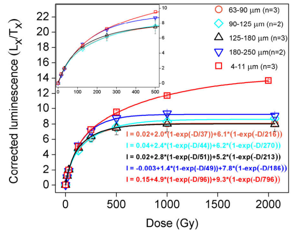
Fig. 4. SAR dose response curves for doses up to 2000 Gy for aliquots of 4–11, 63–90, 90–125, 125–180 and 180–250 \mu\text{m} quartz extracted from sample M#6#. The inset shows an enlargement for the dose region up to 500 Gy. The number of aliquots used for each fraction and the equations used to fit the curves are also indicated.
