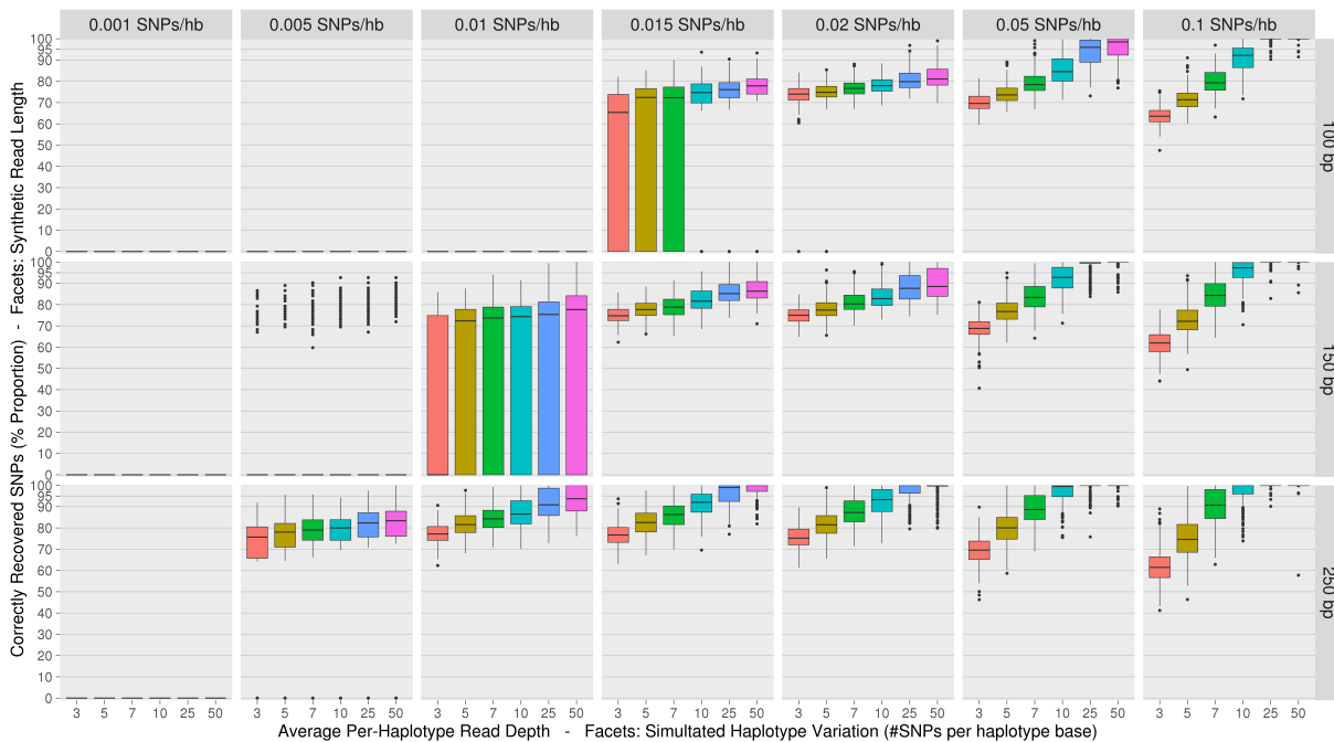
Figure 1: Boxplots summarising the proportion of variants on an input haplotype correctly recovered (y-axes) from groups of synthetic metahaploomes by Gretel . Single boxplots present recoveries from a set of five metahaploomes generated with some per-haplotype mutation rate (column facets), over 10 different synthetic read sets with varying read length (row facets) and per-haplotype read depth (colour fill). Each box-with-whiskers summarises the proportion of correctly recovered variants over the 250 best recovered haplotypes (yielded from 50 Gretel runs (5 metahaploome replicates \times 10 read sets), each returning 5 best outputs). We demonstrate better haplotype recoveries can be achieved with longer reads and more dense coverage, as well as the limitations of recovery on data exhibiting fewer SNPs/hb. This figure may be used as a naive lookup table to assess potential recovery rates for one’s own data by estimating the level of variation, with the average read length and per-haplotype depth.
