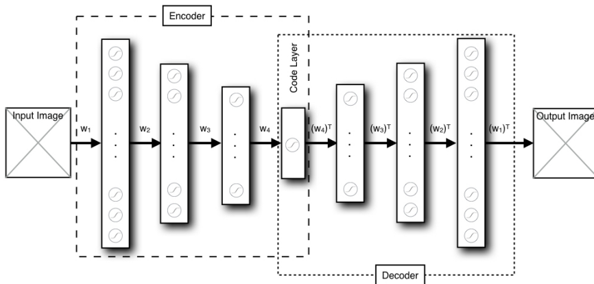
Figure 4: Schematic architecture of an AutoEncoder (AE).
