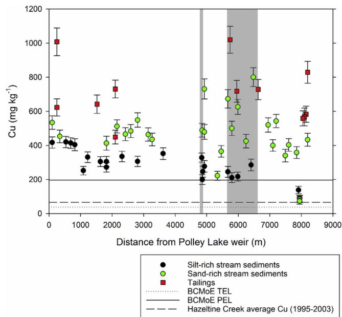
Fig. 3. pXRF-derived Cu concentrations of sediments in Hazelatine Creek sampled on August 1st, 2014. Dotted line and solid line represent British Columbia Ministry of Environment (BCMoE) Threshold Effect Limits (TEL) and Predicted Effect Limits (PEL), respectively (British Columbia Ministry of Environment (BCMoE), 2015). The dashed line represents the Hazelatine Creek average Cu concentration from 1995 to 2003 (Golder Associates Ltd, 2015). Grey vertical bars represent the locations of two bedrock canyons at 4800–4900 m and 5600–6600 m below Polley Lake weir.
