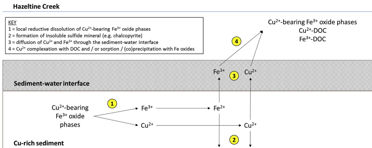
Fig. 7. Conceptual model of Cu transport and cycling in the Hazeltine Creek watershed following the mine tailings spill. A = Polley Flats; B = streambed sediments. *Recent evidence suggests oxidation of chalcopyrite may directly yield Fe 3+ (Pearce et al., 2006).
