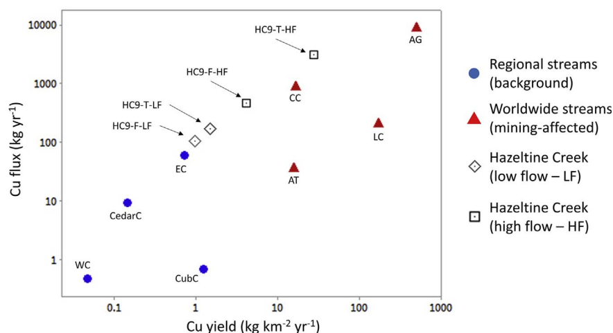
Fig. 8. Cu flux and yield for Hazeltine Creek, regional streams (background) and worldwide streams (mining-affected). Note the logarithmic axes. Hazeltine Creek: HF = high flow; LF = low flow; T = total load; F = filtered load. Regional streams: WC = Winkley Creek; CedarC = Cedar Creek; CubC = Cub Creek; EC = Edney Creek. Worldwide streams: AT = Afon Twymyn (Wales) (Byrne et al., 2013); LC = Lion Creek (USA) (Byrne et al., 2017); CC = Cement Creek (USA) (Runkel et al., 2016); AG = Afon Goch (Wales) (Mayes et al., 2010).
