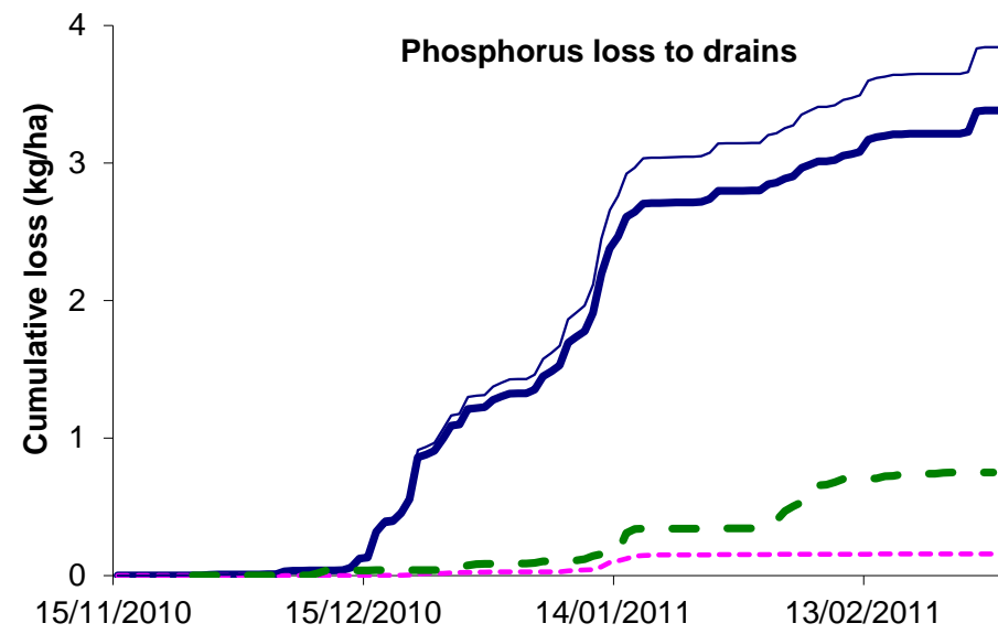
Fig.4. Cumulative losses of contaminants at Welsh and Scottish sites over two winters
