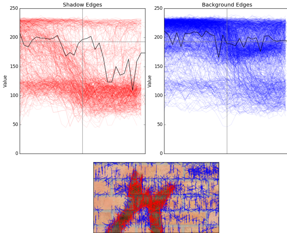
Figure 6: Top left: The brightness profile across lines normal to a shadow edge; Top right: The brightness profile of non-shadow edges. Both of these plots have the mean brightness profile superimposed in black. Bottom: the image from which edge normals were drawn, with normals superimposed in blue. These show that the profiles of shadow edges are demonstrably different to edges detected in non-shadow “background” regions.
