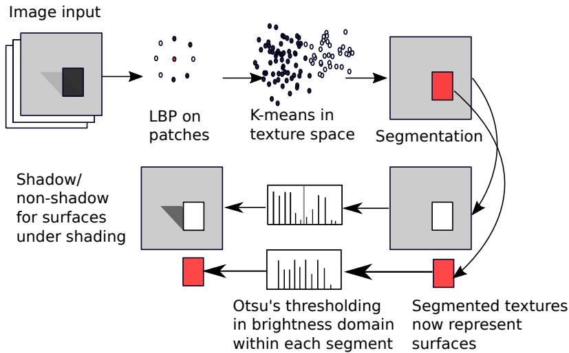
Figure 2: A graphical overview of our texture segmentation approach.
