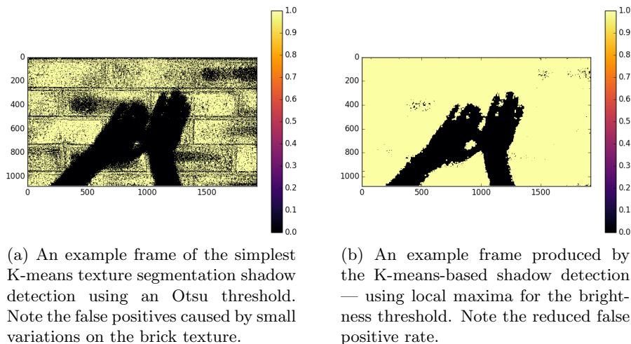
Figure 3: Two frames showing the progression of the K-Means/Otsu algorithm.
