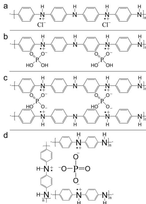
Figure 3. The molecular configurations of polyaniline (a) and three possible molecular configurations of the H 3 PO 4 doped polyaniline (b), (c),(d).
